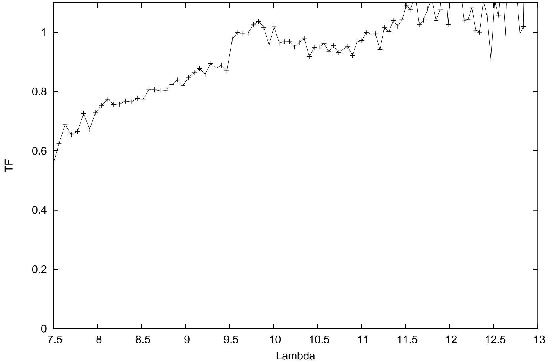
calHIP9884_flux-0.75397_diam7.42869_r.MIDI.2011-12-04T01_18_09.113_K0J3
