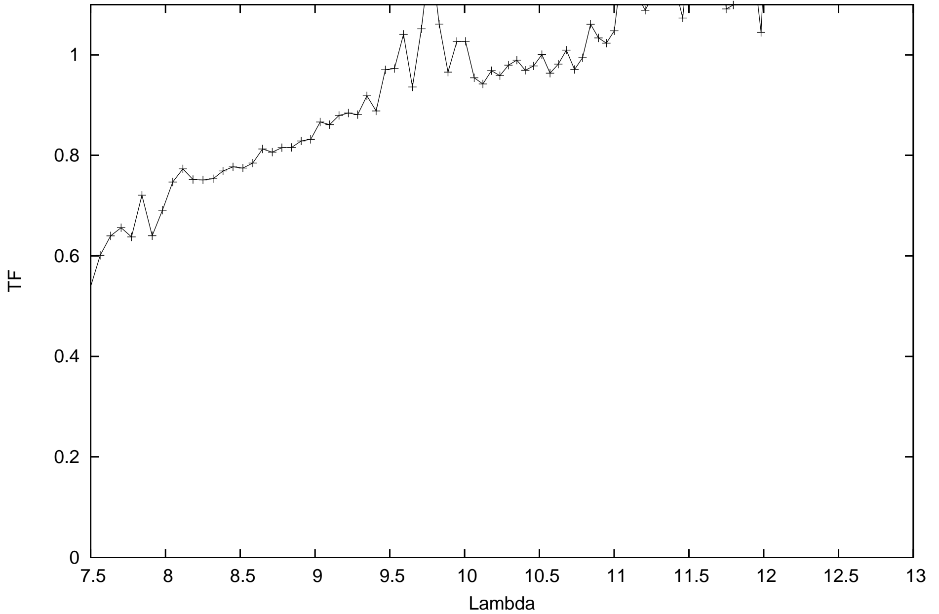
calHIP9884_flux-0.75397_diam7.42869_r.MIDI.2011-12-04T01_00_19.113_K0J3
