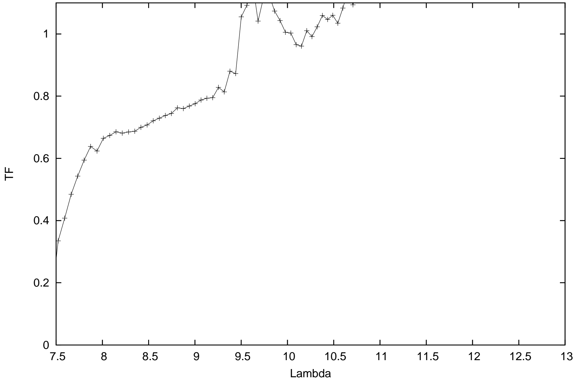
calHIP30438_flux-1.50235_diam6.87_r.MIDI.2011-12-04T09_01_09.000_G1J3
