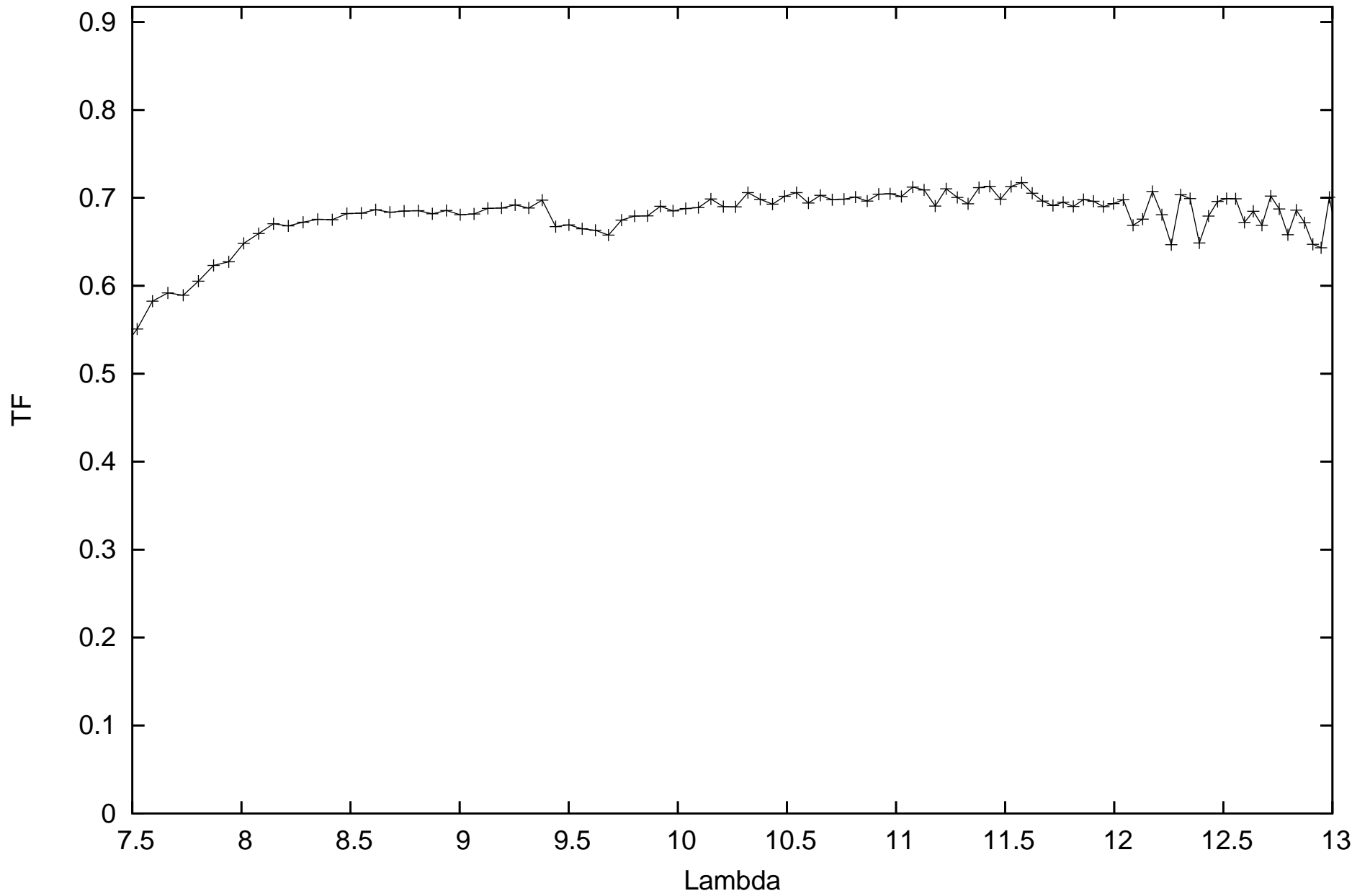
calHD48915_flux-1.39_diam6.09_r.MIDI.2011-12-04T07_04_00.000_K0J3
