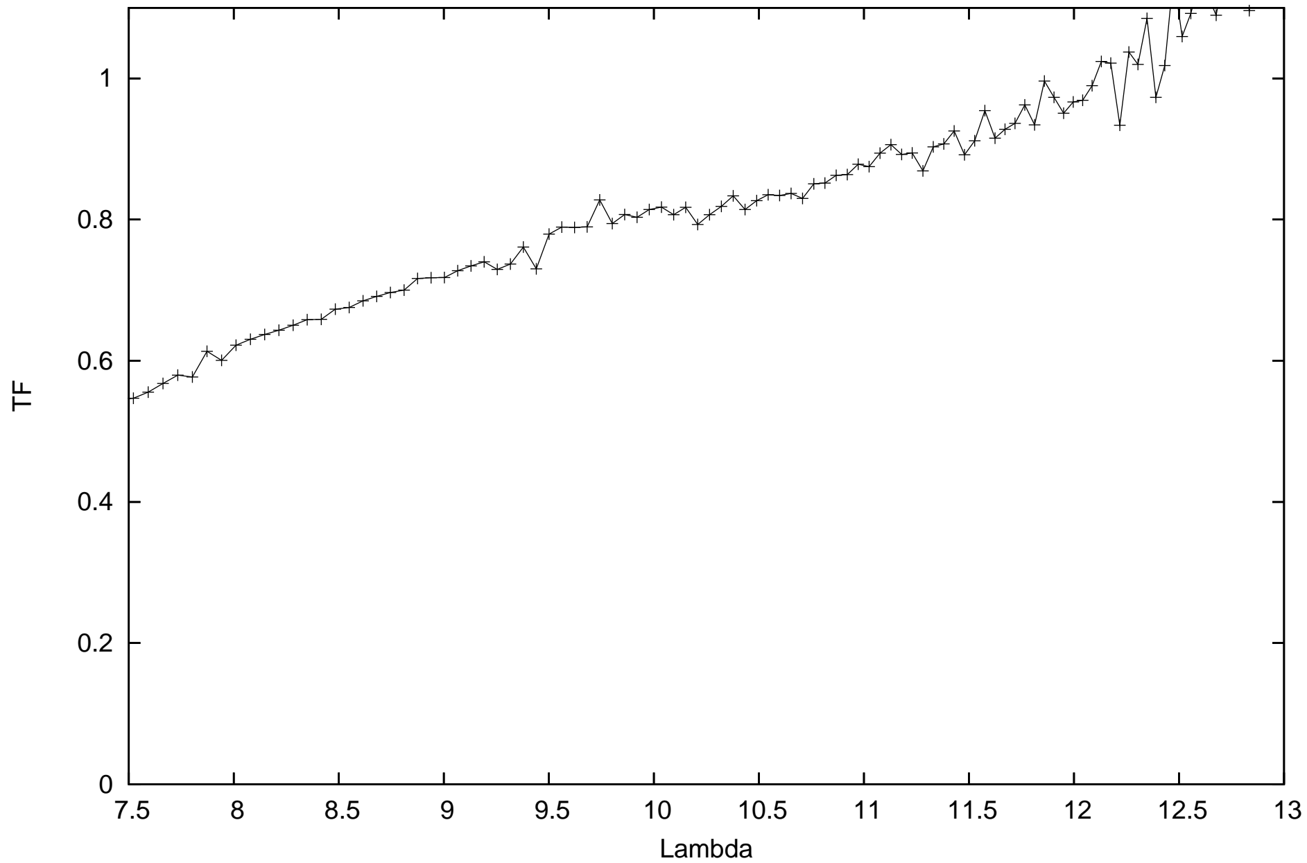
calHD20720_flux-1.53_diam10.14_r.MIDI.2011-11-16T03_10_56.000_K0I1
