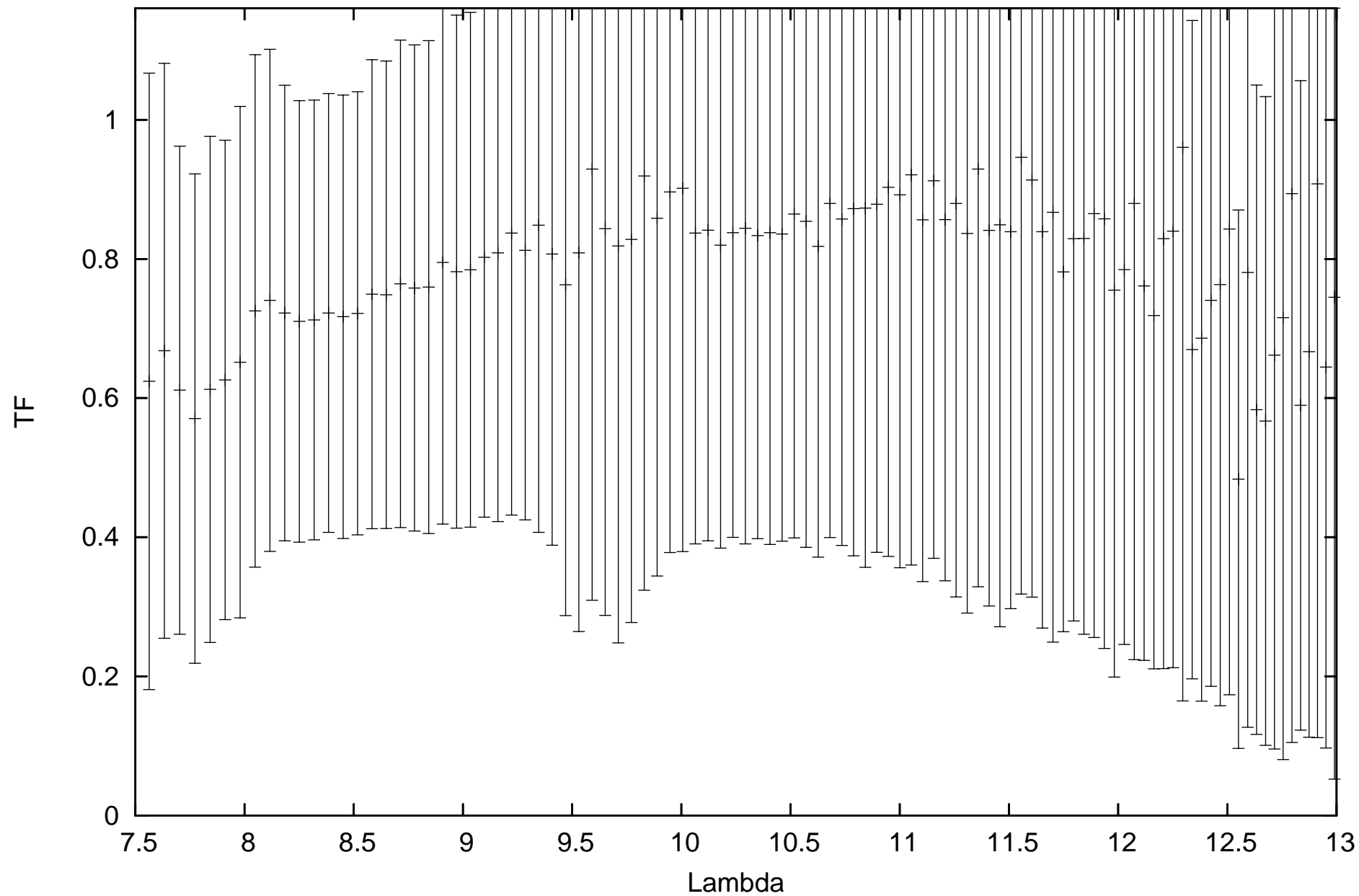
calHIP9884_flux-0.75397_diam7.42869_r.MIDI.2011-11-15T03_51_32.113_K0I1
