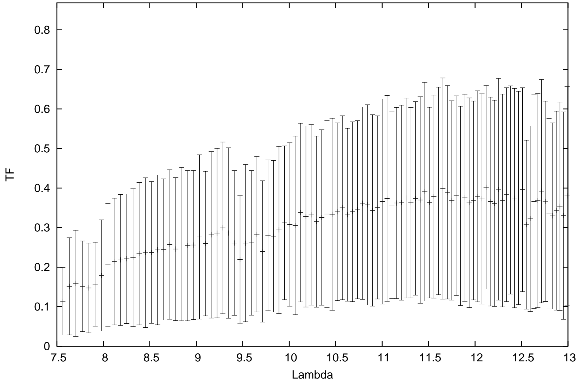
calHD167618_flux-1.82_diam11.66_r.MIDI.2011-11-10T23_37_04.970_K0I1
