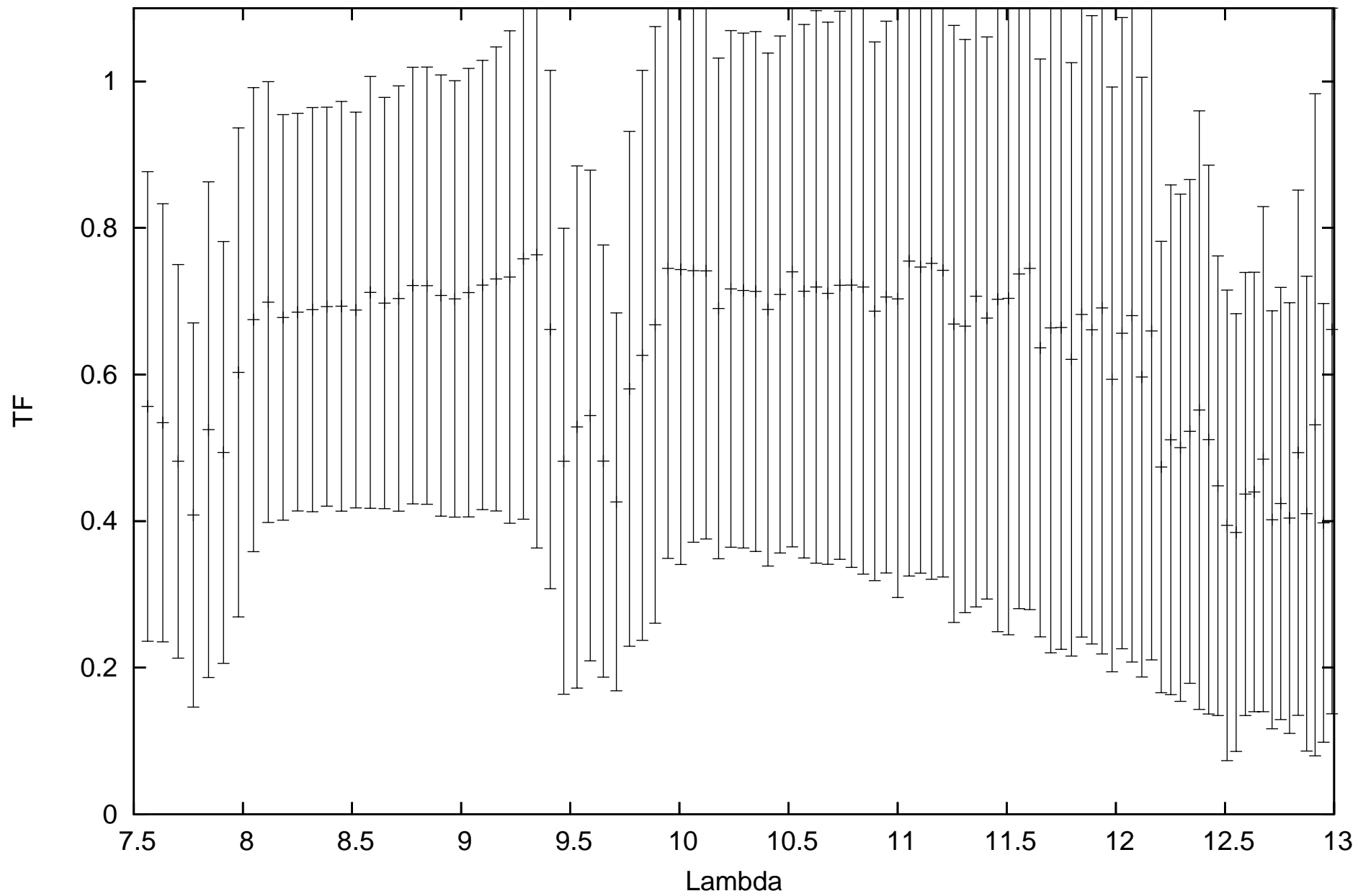
calHIP89931_flux-0.511_diam5.87_r.MIDI.2011-11-05T00_31_29.293_H011
