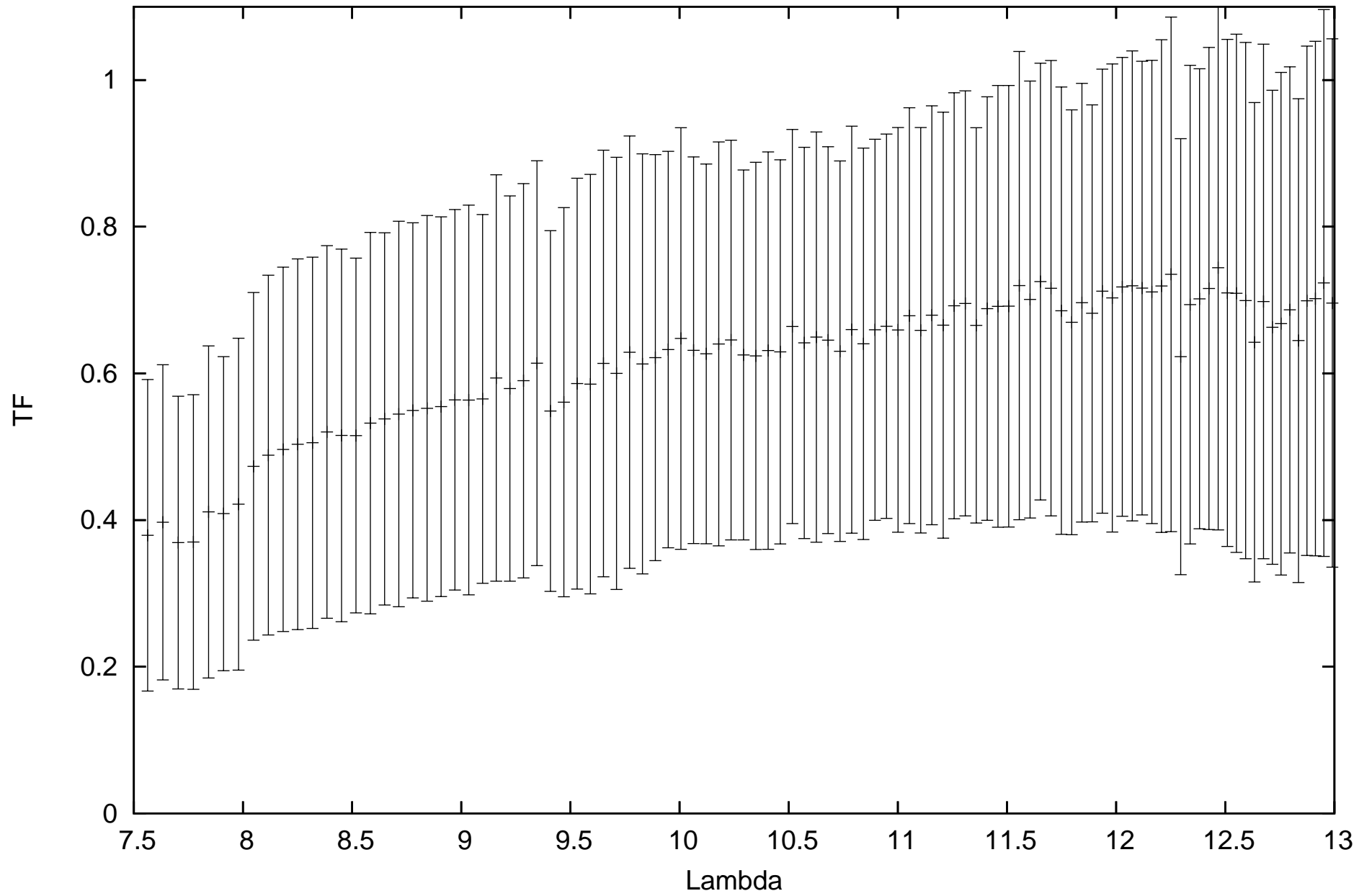
calHD167618_flux-1.82_diam11.66_r.MIDI.2011-11-04T23_51_17.135_H011
