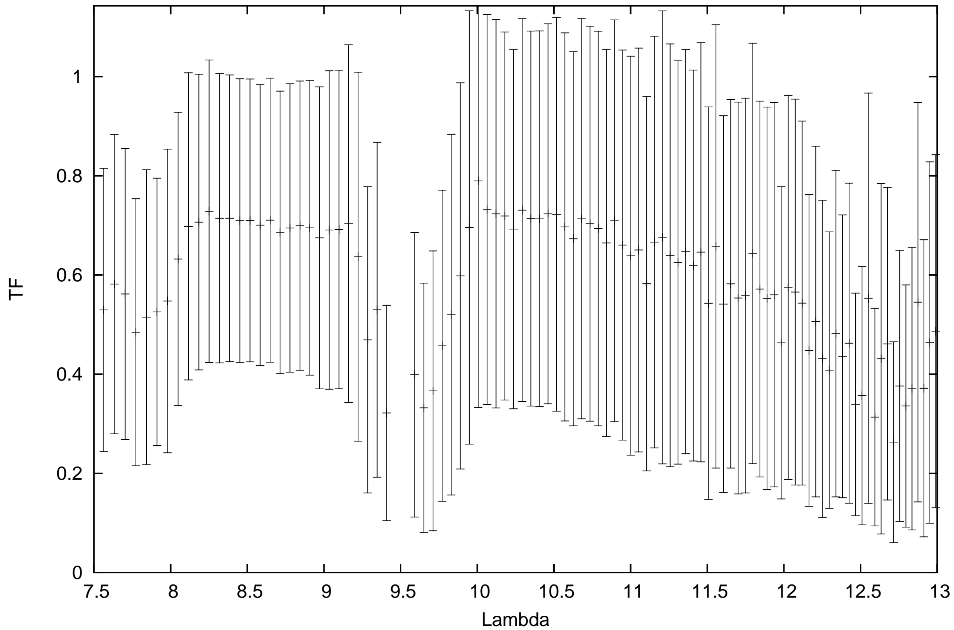
calHIP89931_flux-0.511_diam5.87_r.MIDI.2011-11-03T23_48_40.969_G111
