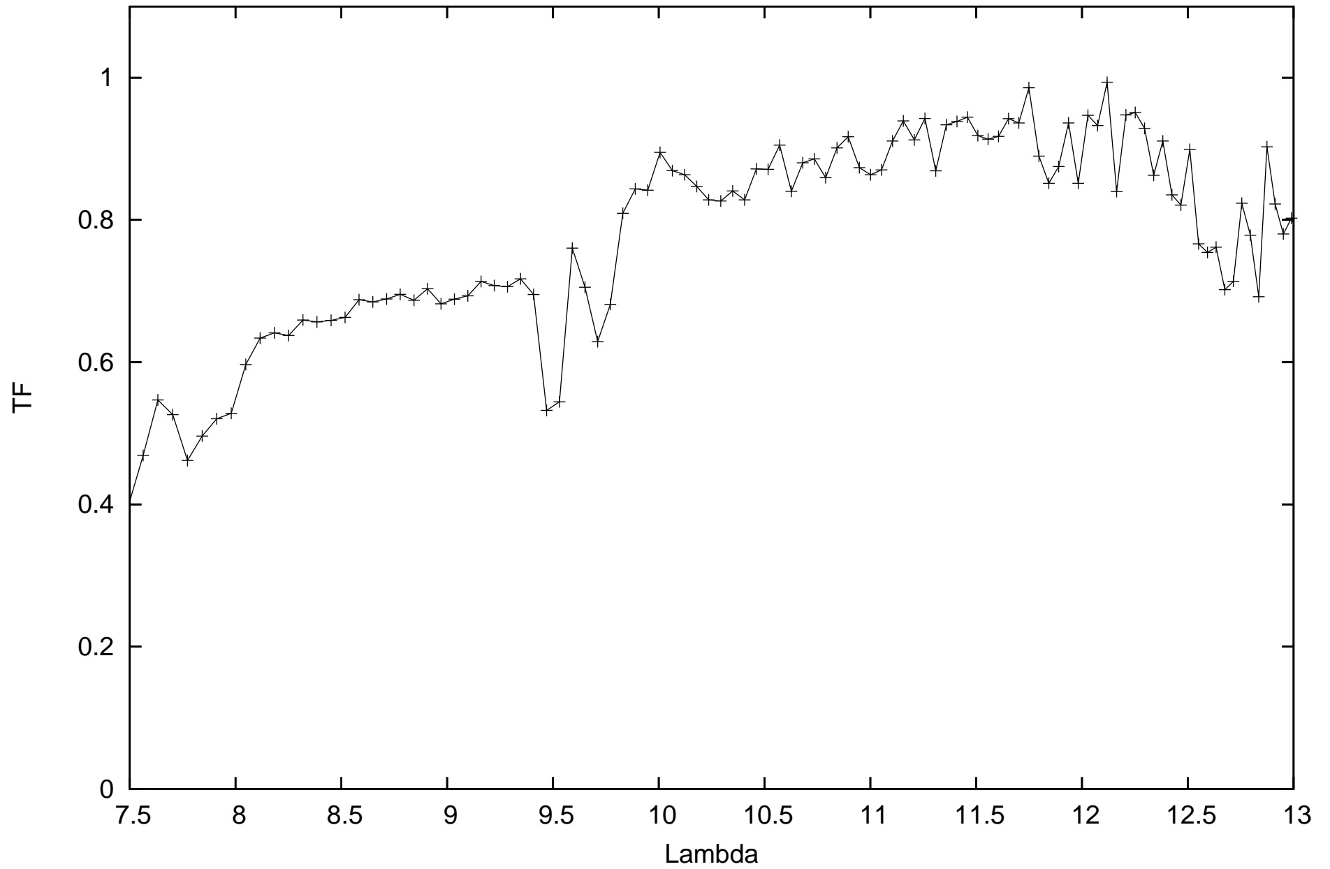
calHIP46701_flux-0.68631_diam6.952948_r.MIDI.2011-11-04T08_20_17.128_H011
