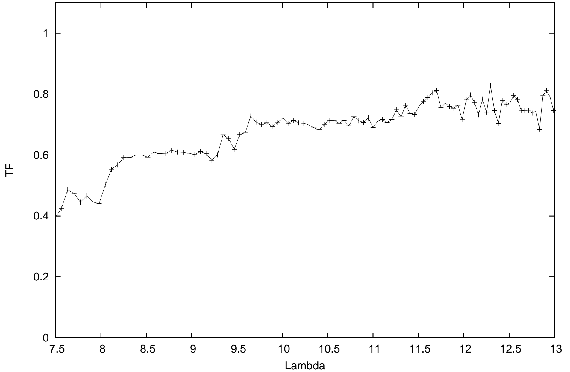
calHIP14135_flux-1.95419_diam12.27_r.MIDI.2011-11-04T05_41_47.933_H011
