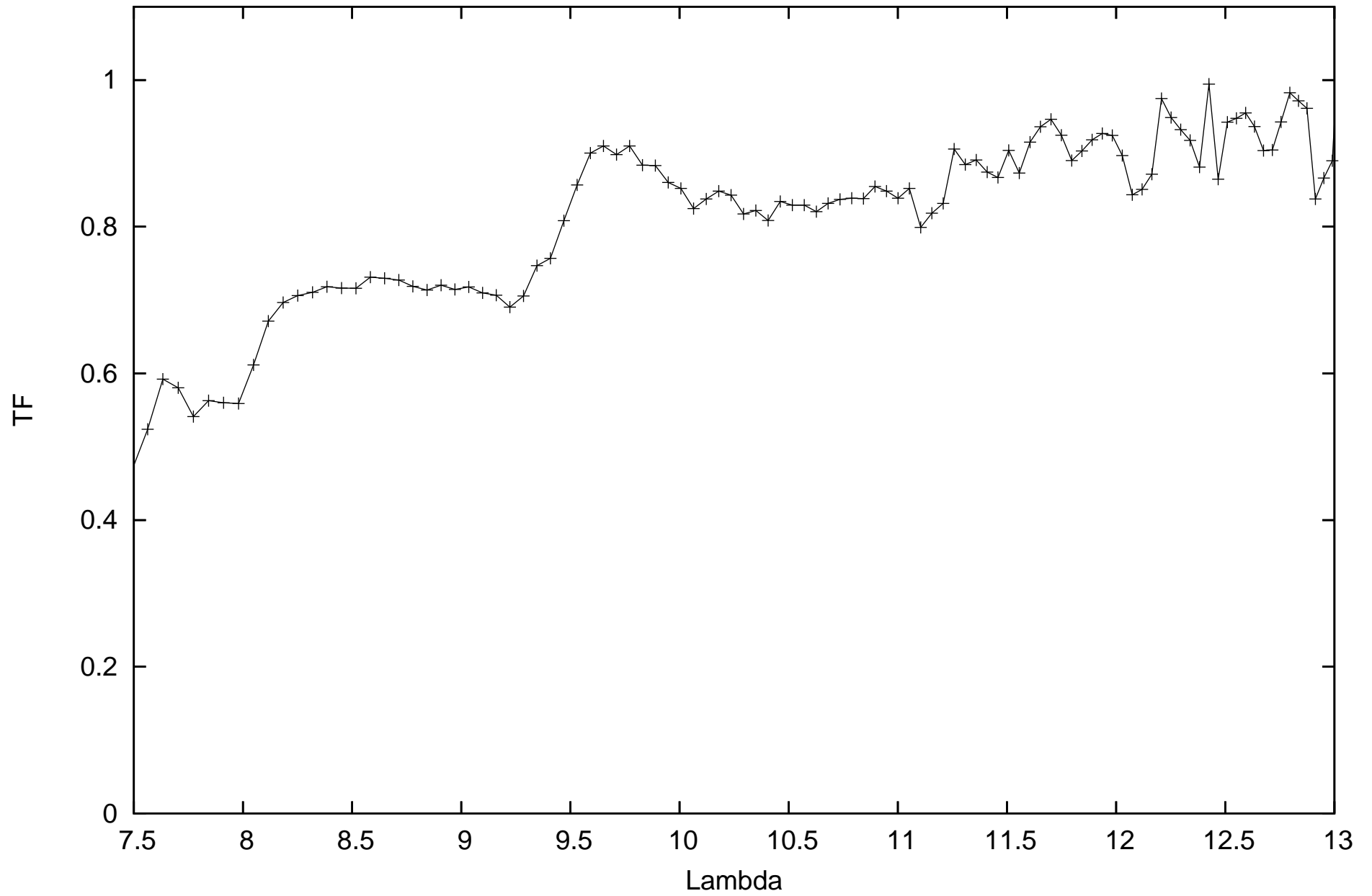
calHIP14135_flux-1.95419_diam12.27_r.MIDI.2011-11-04T04_09_23.932_H011
