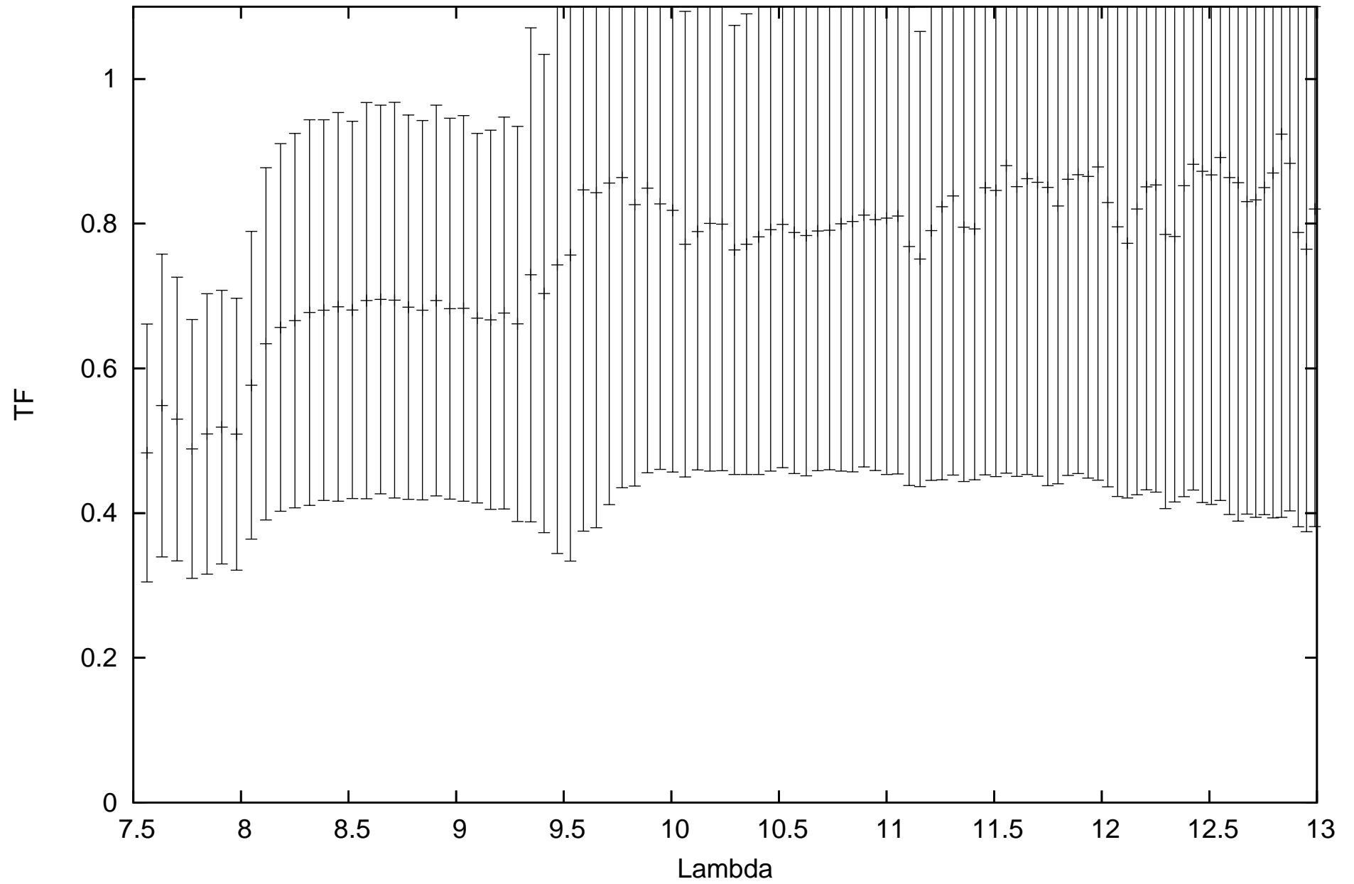
calHIP14135_flux-1.95419_diam12.27_r.MIDI.2011-11-04T03_33_16.135_H011
