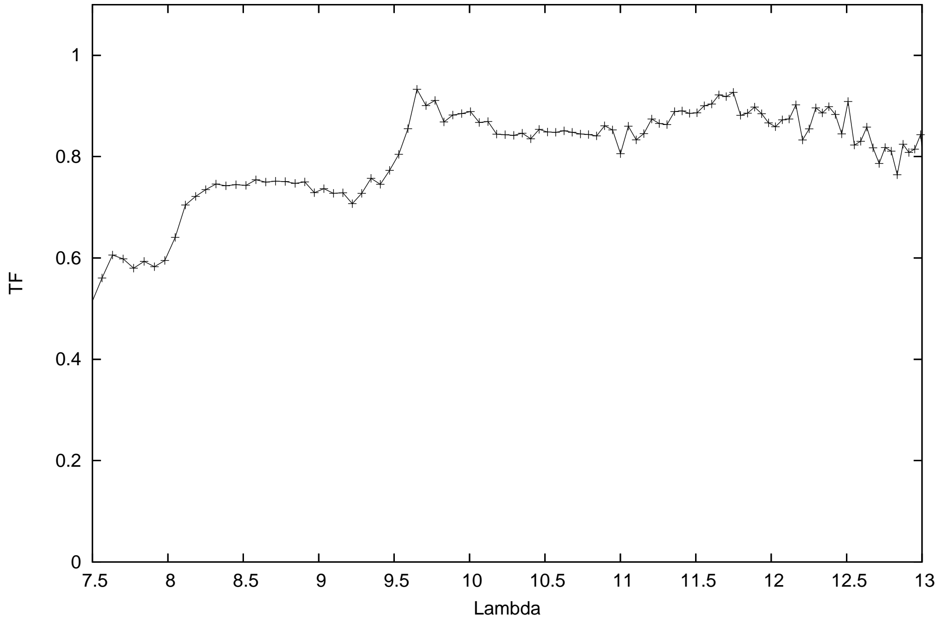
calHD20720_flux-1.53_diam10.14_r.MIDI.2011-11-04T02_37_08.135_H011
