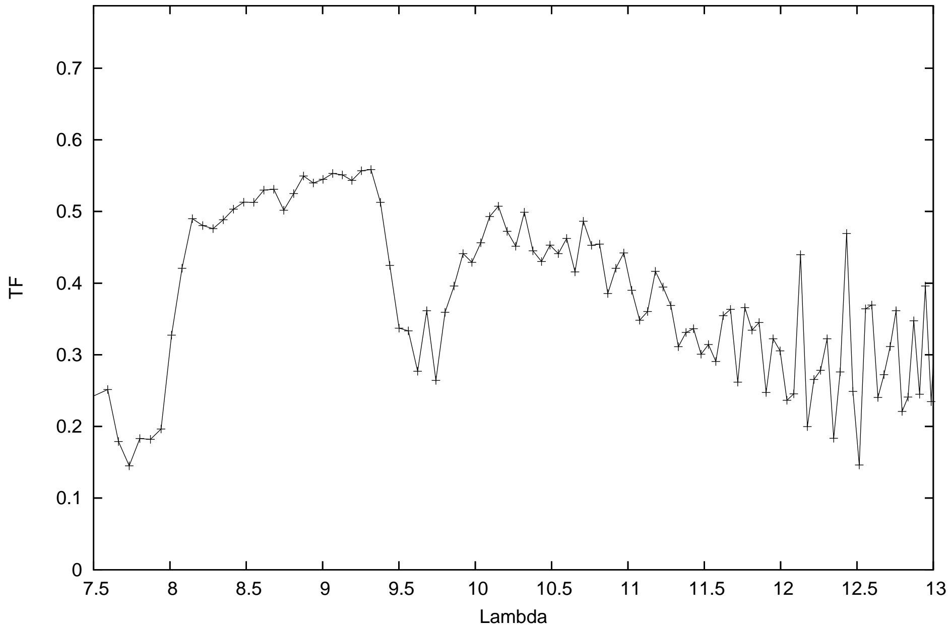
calHIP33160_flux0.496137_diam3.9_r.MIDI.2011-11-01T09_01_21.000_G111
