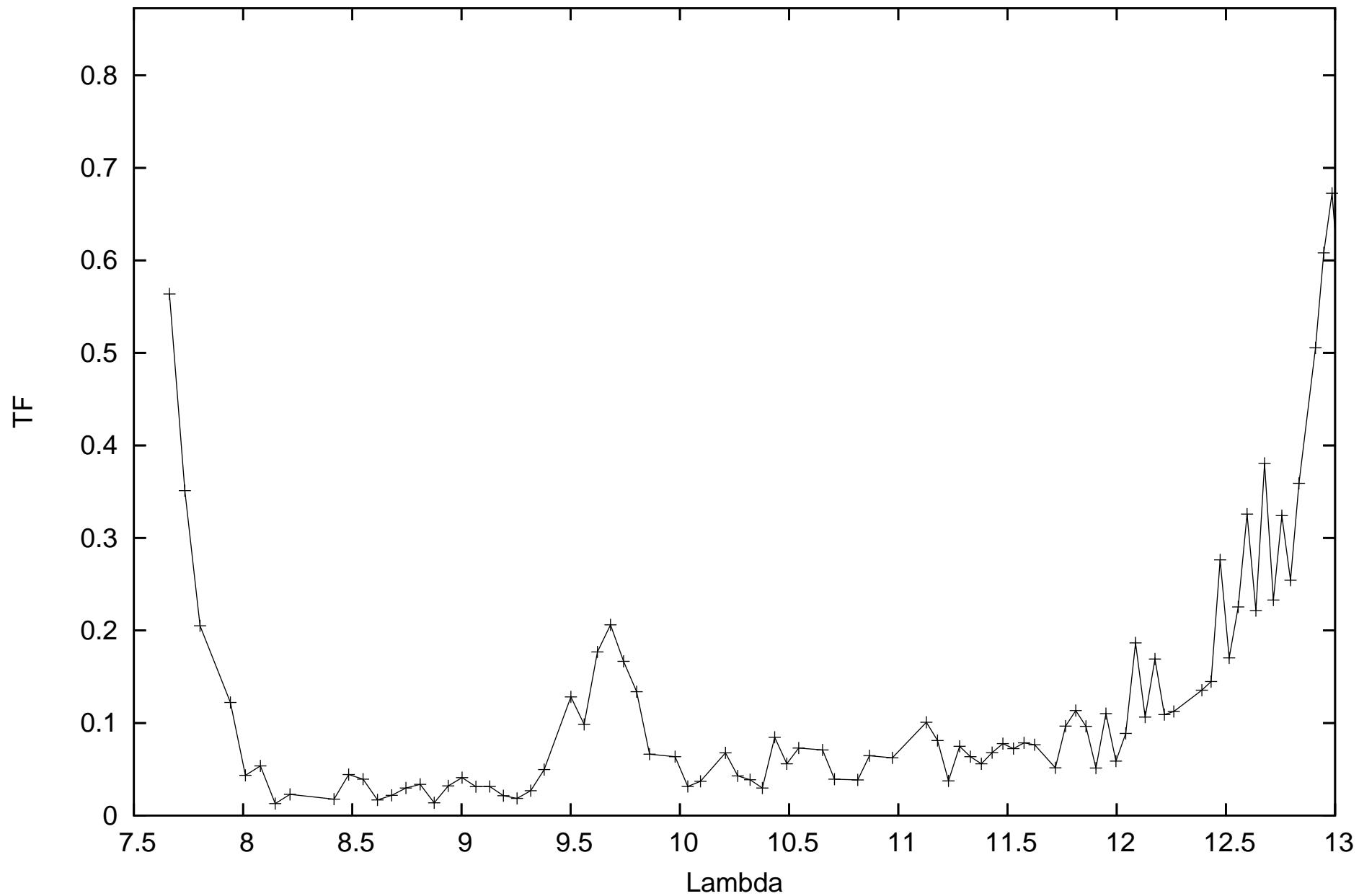
calHIP33160_flux0.496137_diam3.9_r.MIDI.2011-11-01T04_20_10.000_G111
