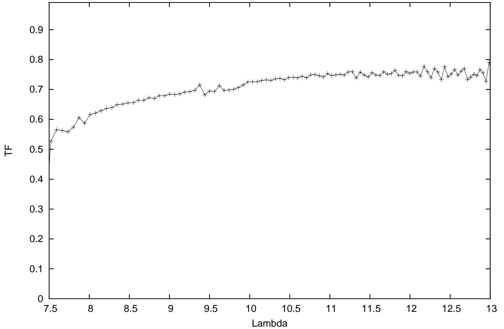
calHIP14135_flux-1.95419_diam12.27_r.MIDI.2011-11-01T03_52_36.000_G111
