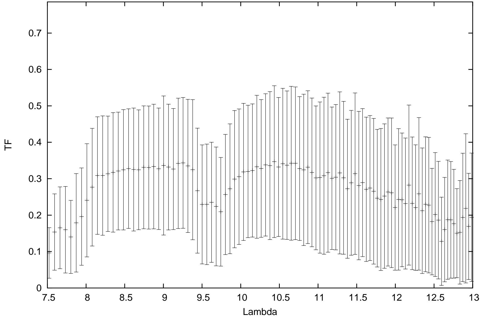
calHD224935_flux-0.85_diam7.24_r.MIDI.2011-11-01T01_44_54.000_K0A1
