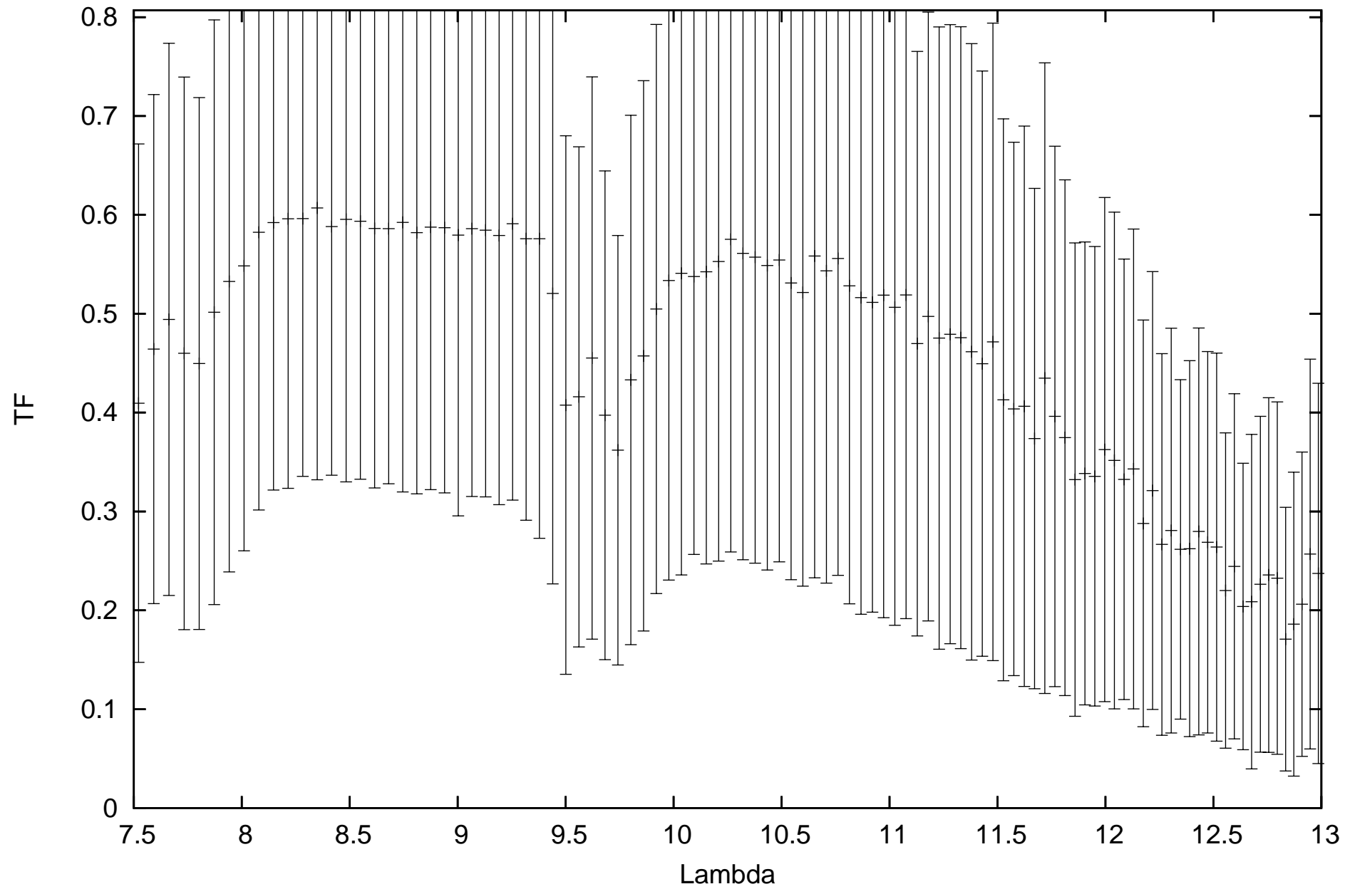
calHIP1170_flux-0.10766_diam5.17_r.MIDI.2011-10-30T03_41_42.000_G1A1
