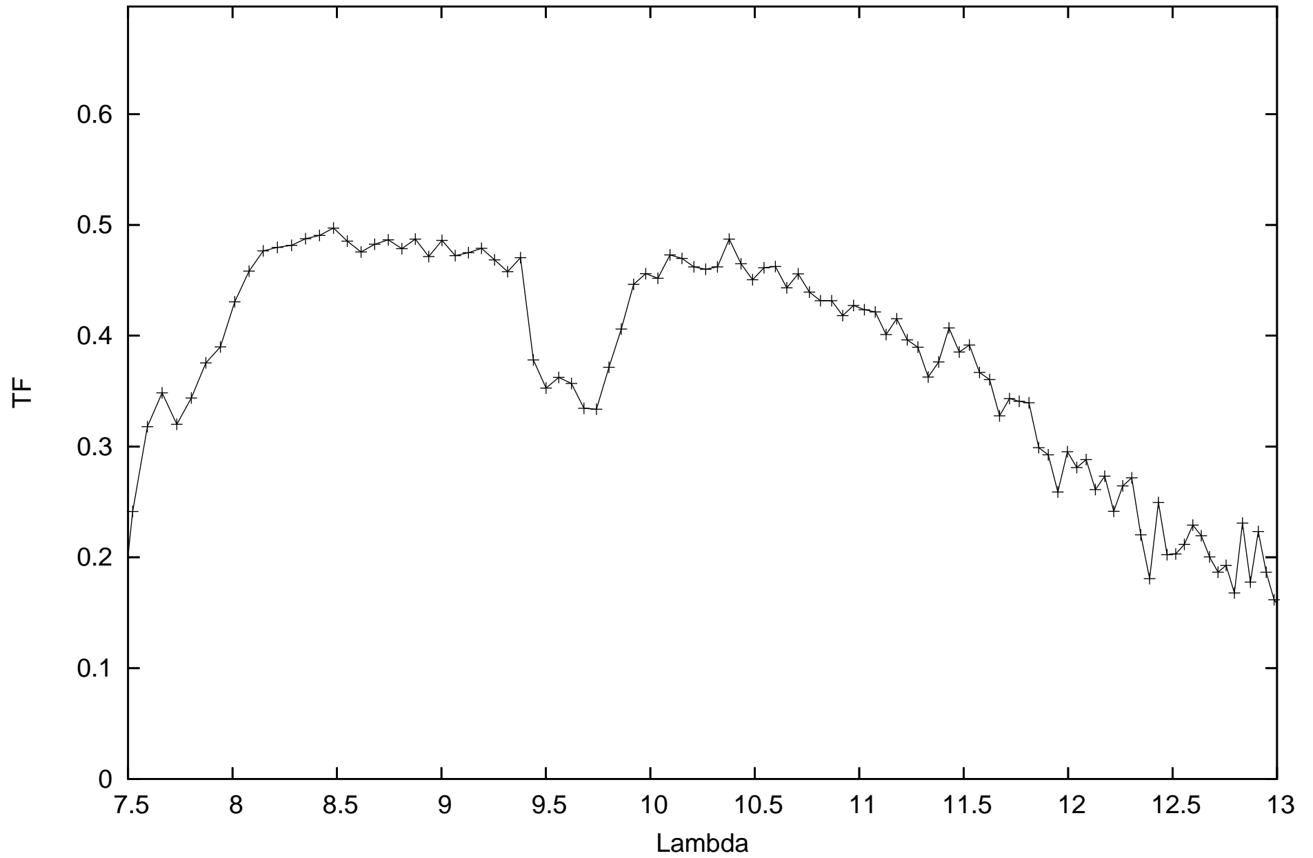
calHIP1170_flux-0.10766_diam5.17_r.MIDI.2011-10-30T02_41_19.000_K0A1
