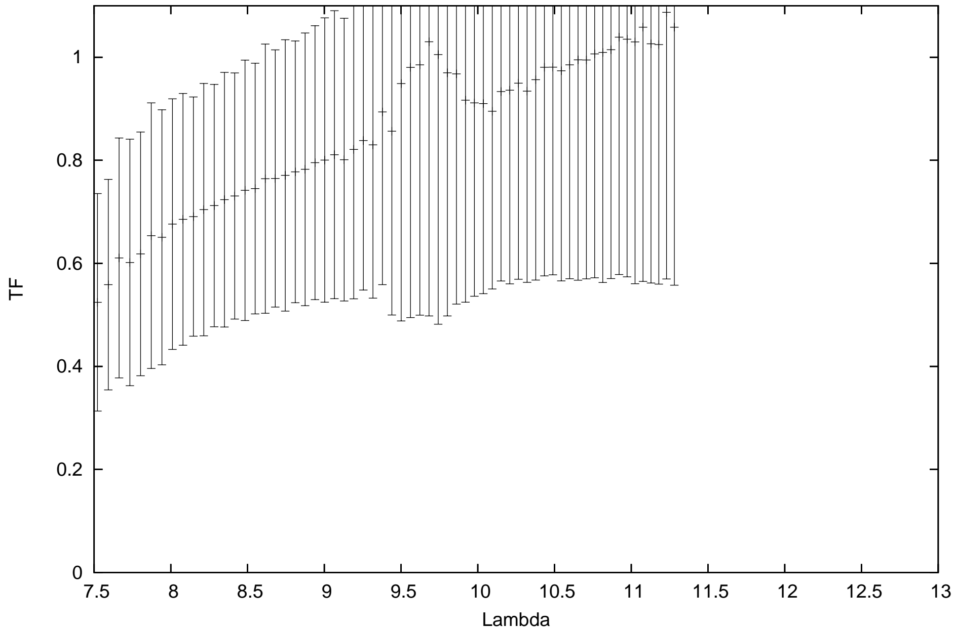
calHD48915_flux-1.39_diam6.09_r.MIDI.2011-10-27T05_08_25.000_K0G1
