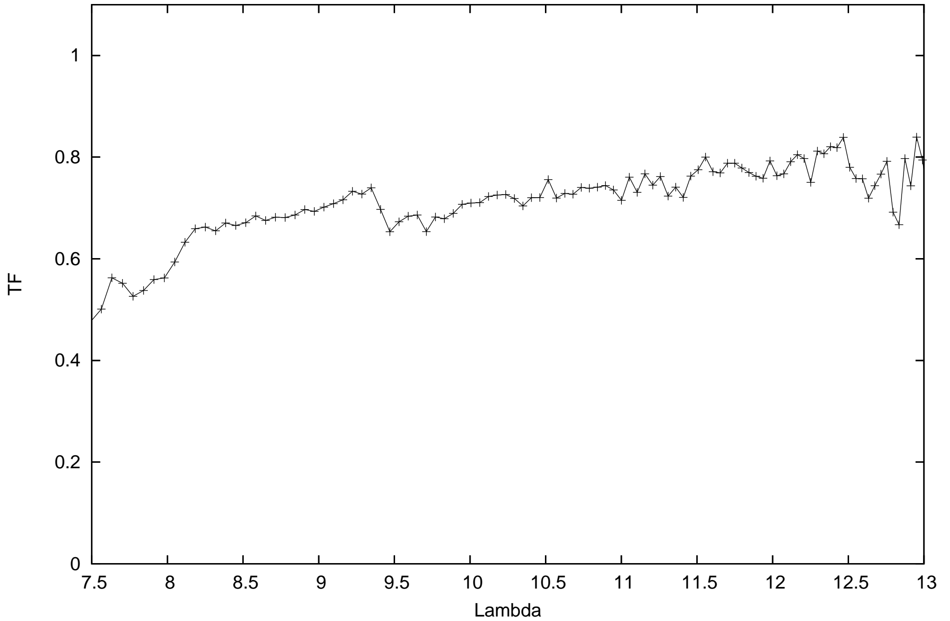
calHD20720_flux-1.53_diam10.14_r.MIDI.2011-10-26T08_03_40.135_D0B2
