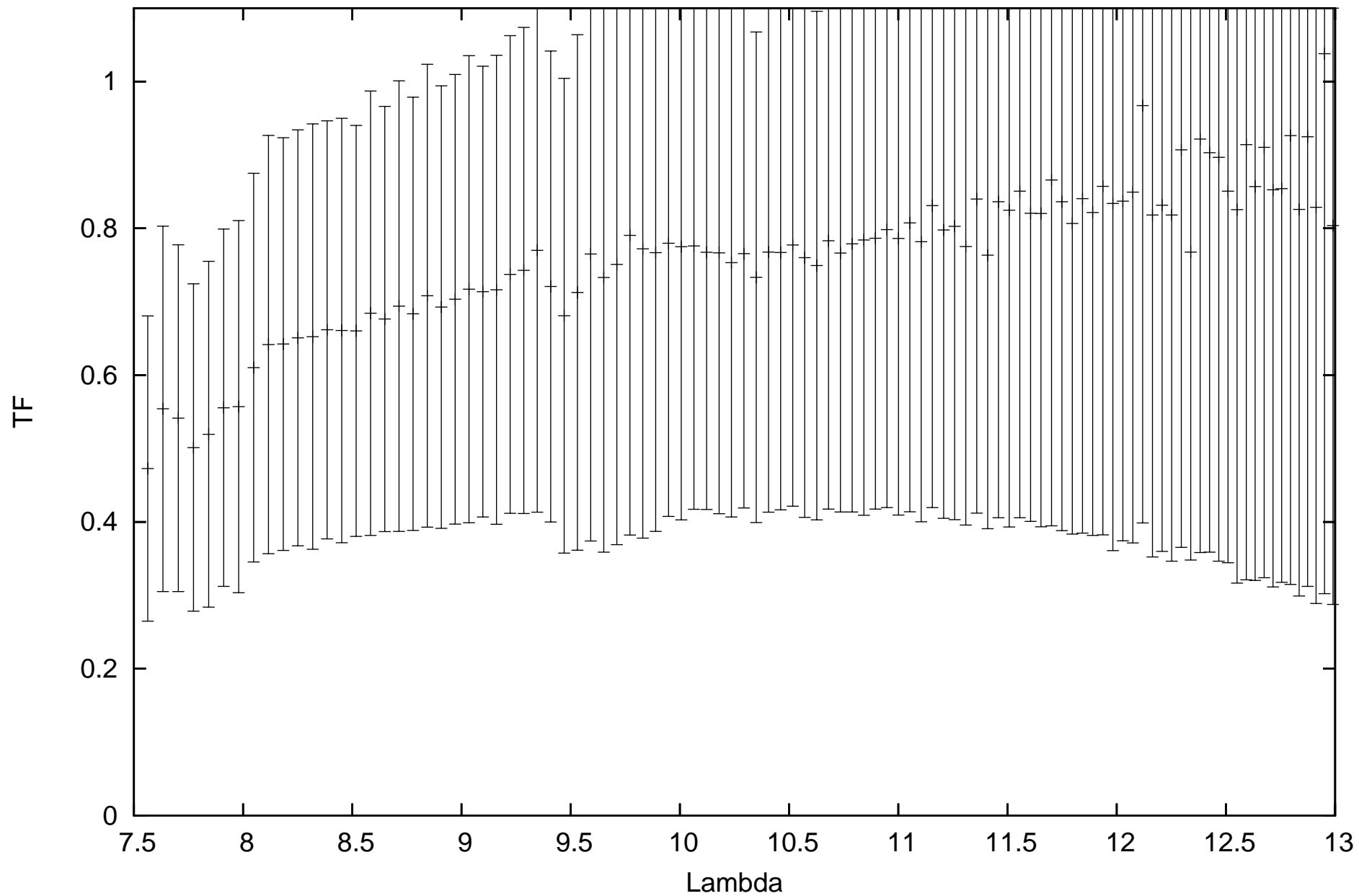
calHIP14135_flux-1.95419_diam12.27_r.MIDI.2011-10-25T08_11_21.939_C1A1
