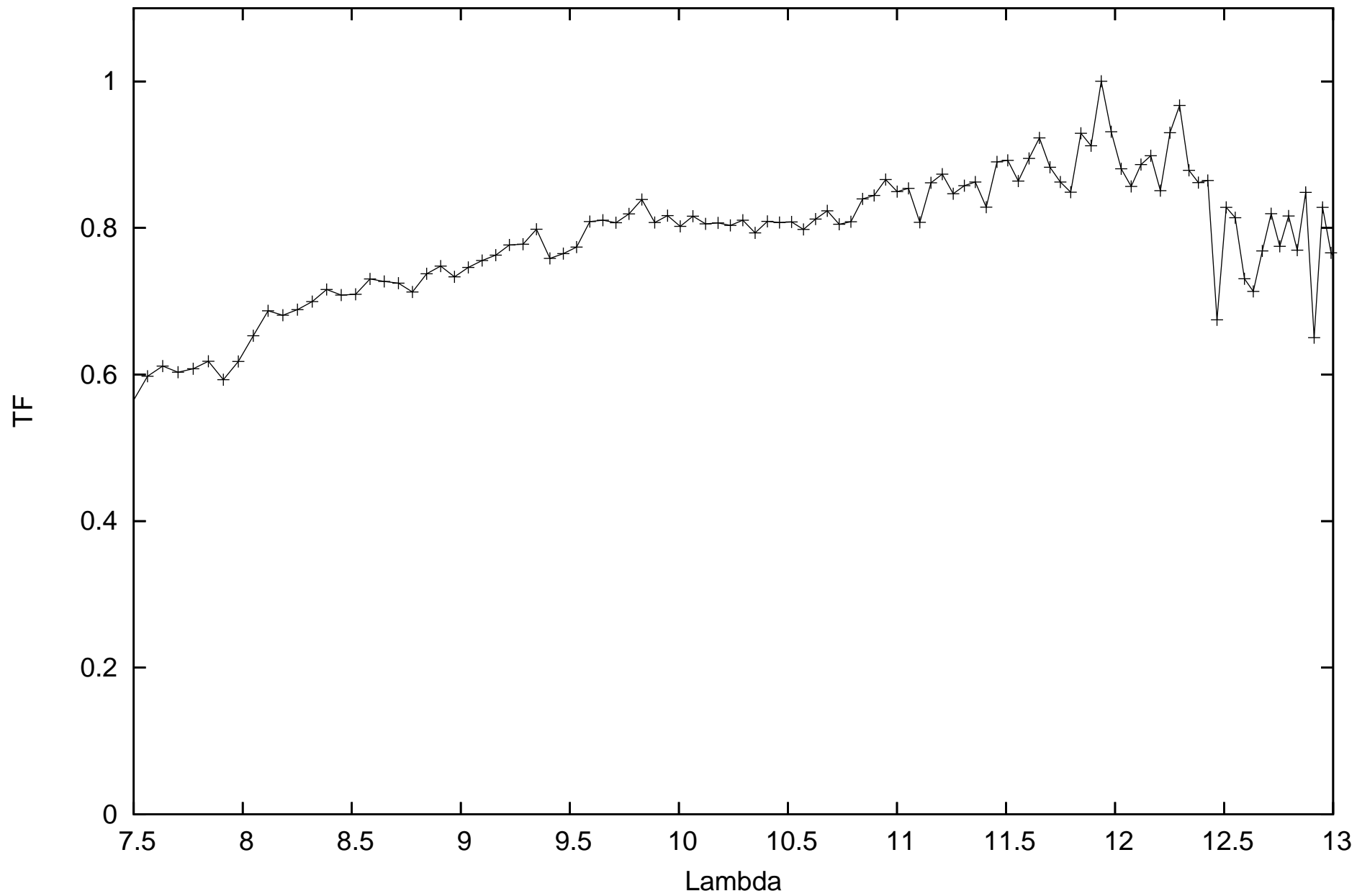
calHIP14135_flux-1.95419_diam12.27_r.MIDI.2011-10-25T05_33_18.135_B2A1
