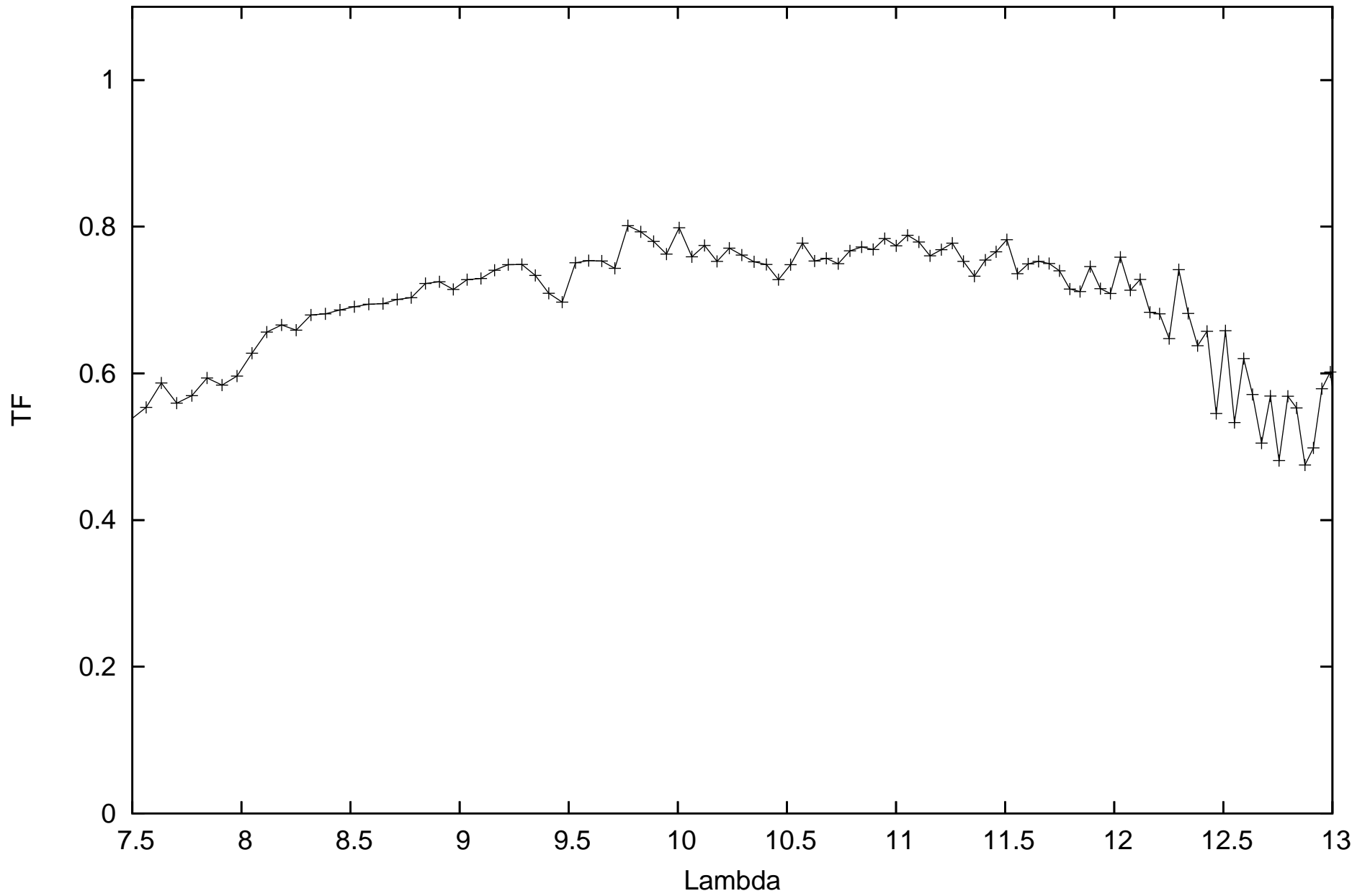
calHIP14135_flux-1.95419_diam12.27_r.MIDI.2011-10-25T04_46_48.970_B2A1
