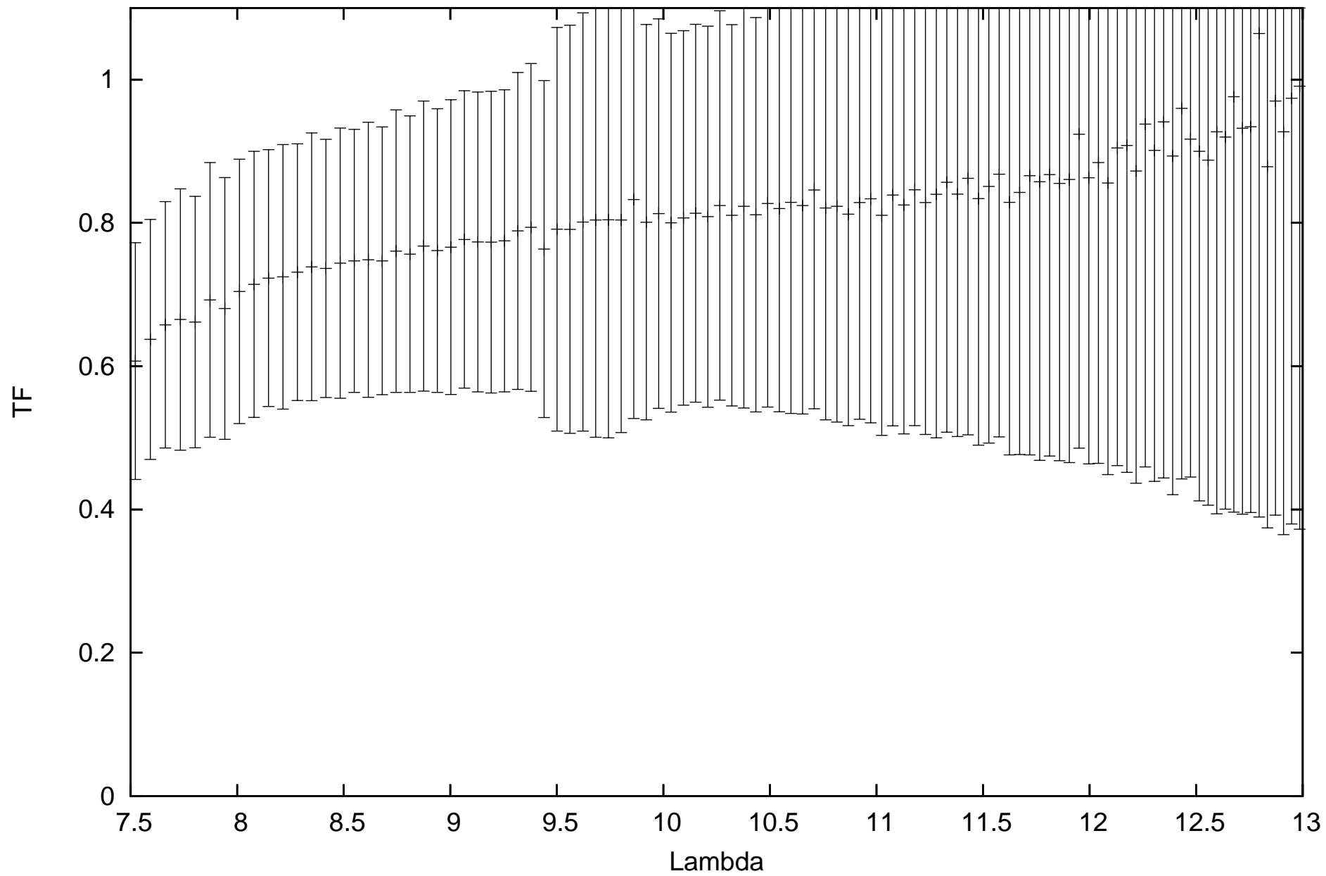
calHD48915_flux-1.39_diam6.09_r.MIDI.2011-10-25T08_52_42.000_C1A1
