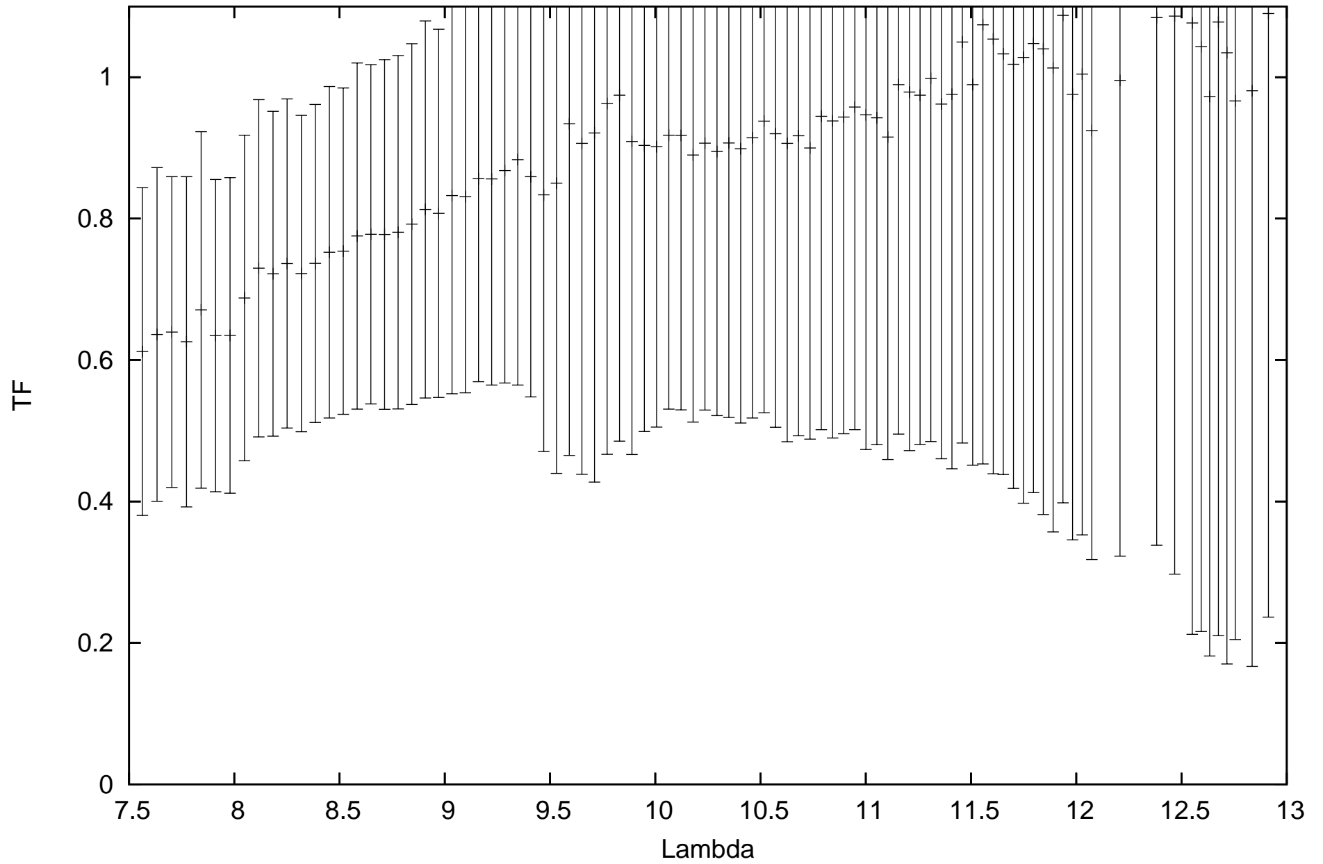
calHD48915_flux-1.39_diam6.09_r.MIDI.2011-10-24T08_02_43.135_D0A1
