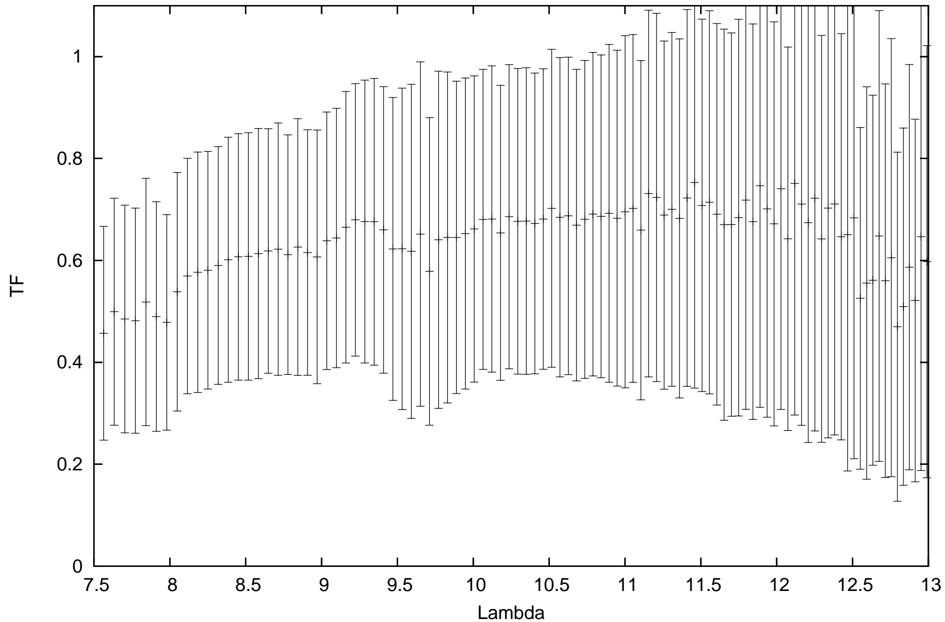
calHD20720_flux-1.53_diam10.14_r.MIDI.2011-10-24T06_16_04.970_D0A1
