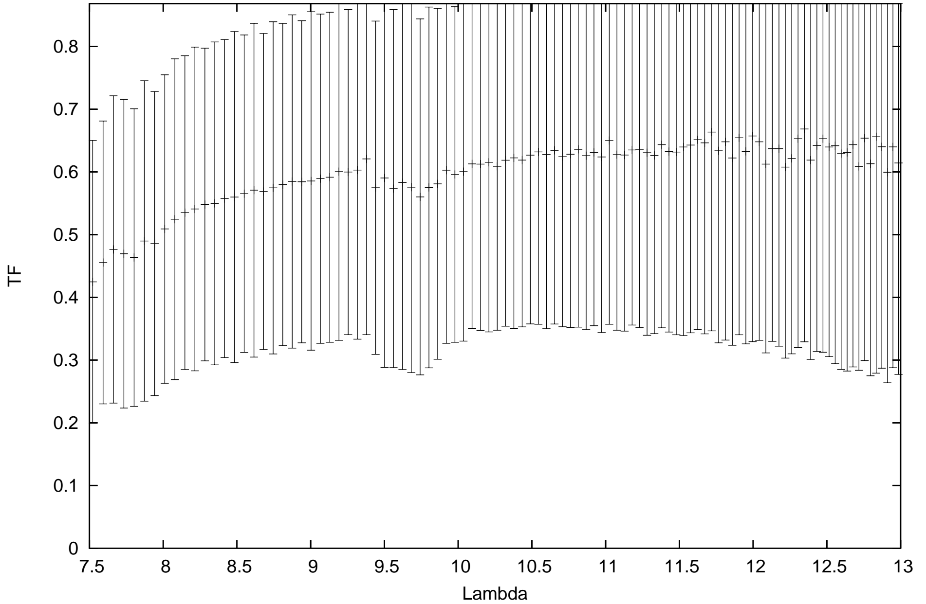
calHIP20324_flux1.95295_diam2.257387_r.MIDI.2011-10-10T06_51_37.000_U1U2
