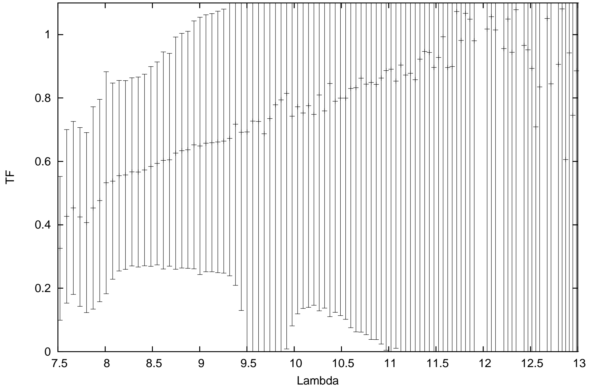
calHIP9884_flux-0.75397_diam7.42869_r.MIDI.2011-10-06T07_58_18.000_J3A1
