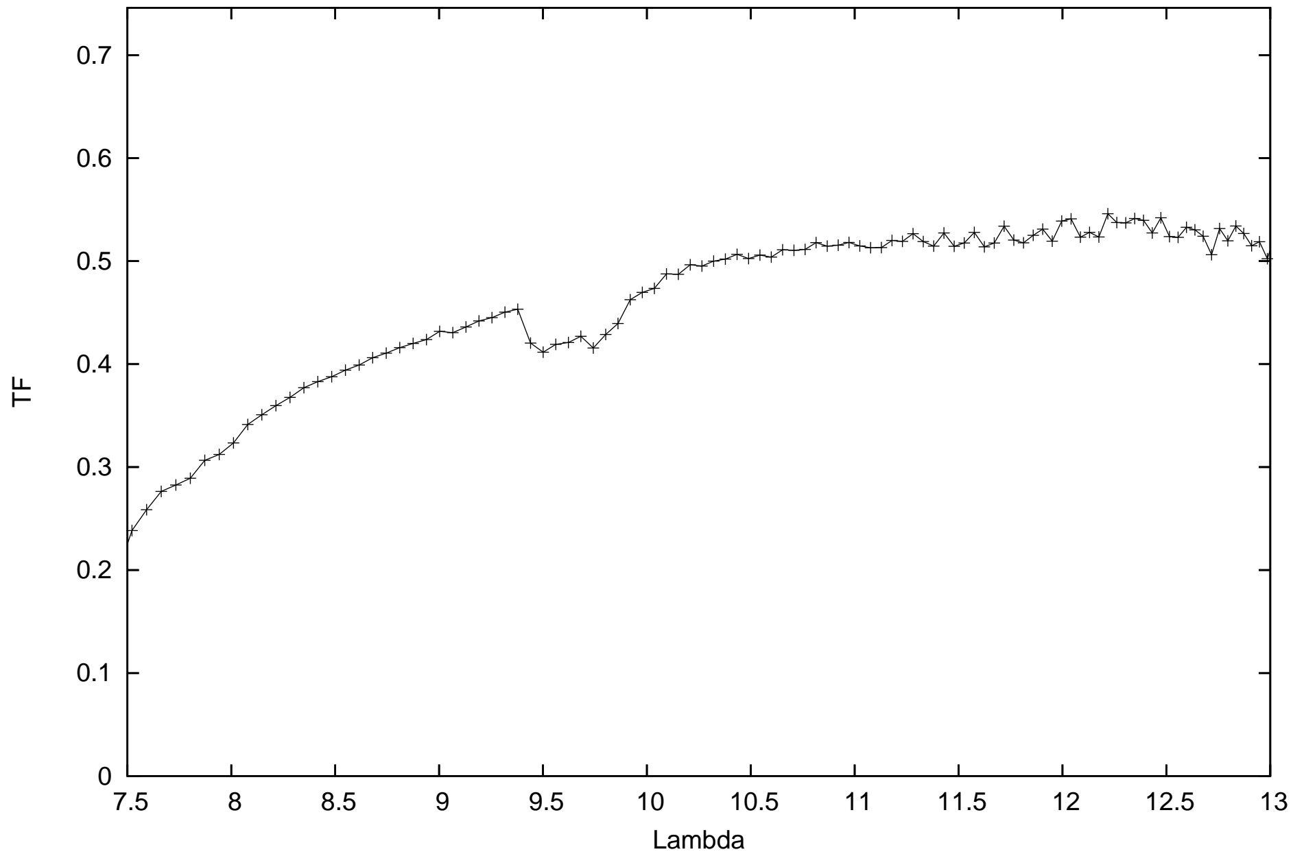
calHD167618_flux-1.82_diam11.66_r.MIDI.2011-10-06T00_20_09.000_K0A1
