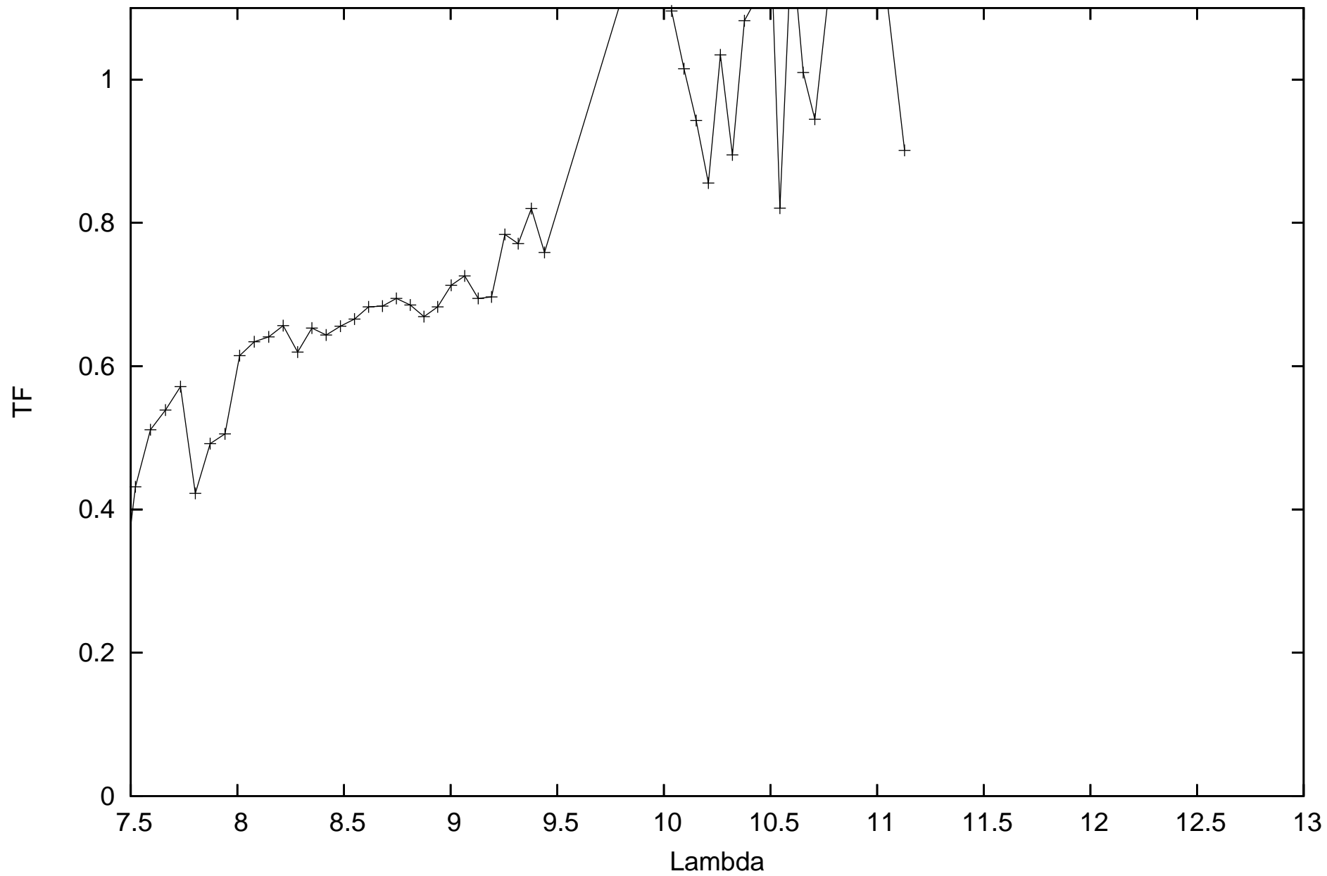
calHIP33357_flux0.277058_diam4.37_r.MIDI.2011-10-05T07_47_20.000_J3A1
