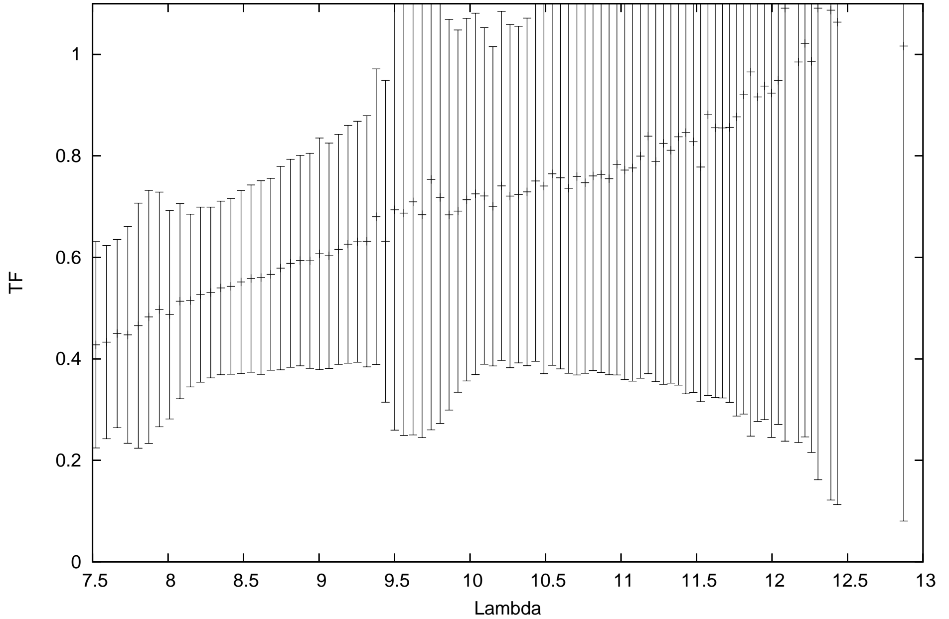
calHD224935_flux-0.85_diam7.24_r.MIDI.2011-10-05T06_19_27.000_A1J3
