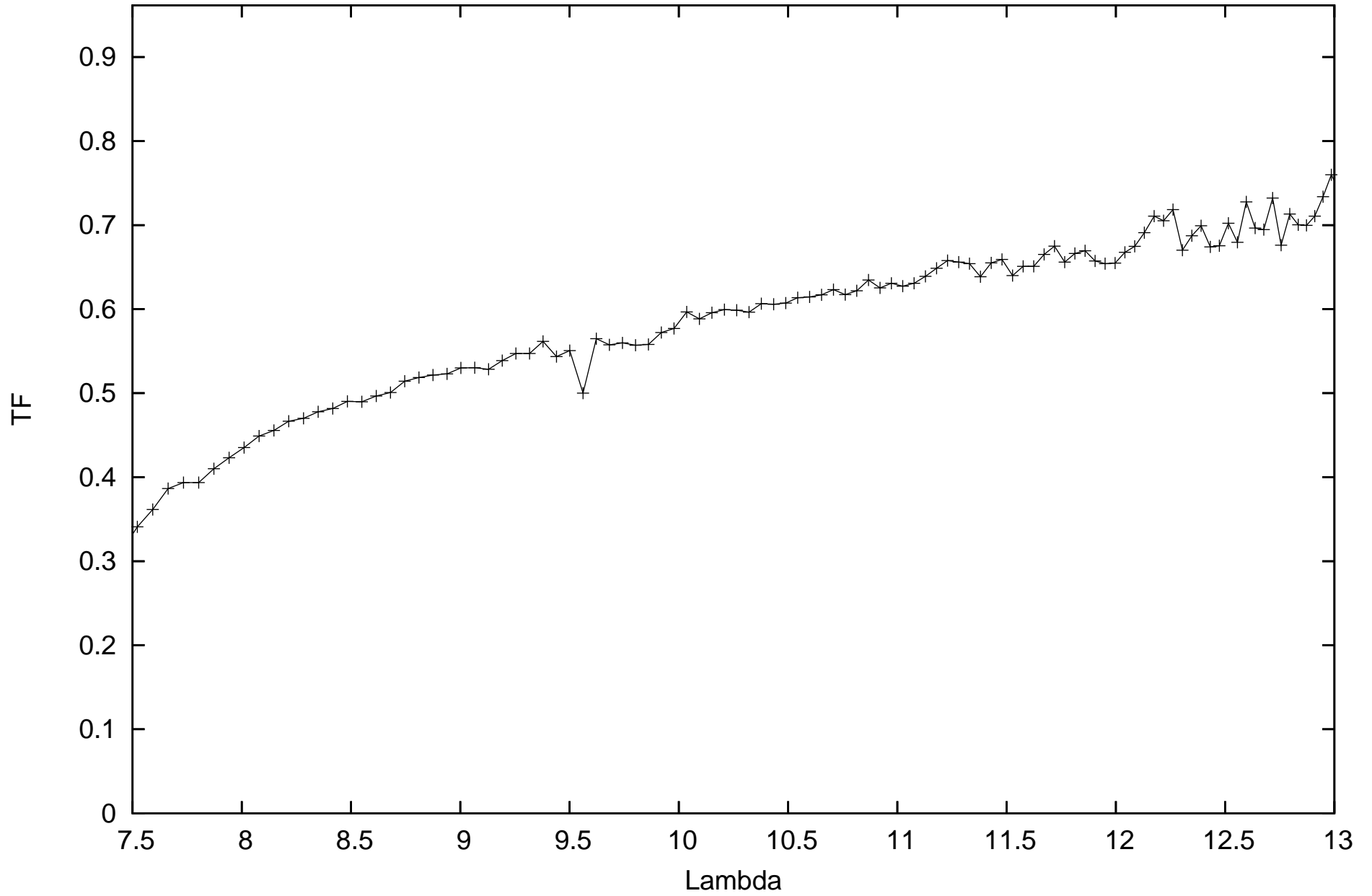
calHIP14135_flux-1.95419_diam12.27_r.MIDI.2011-10-04T07_34_56.000_J3K0
