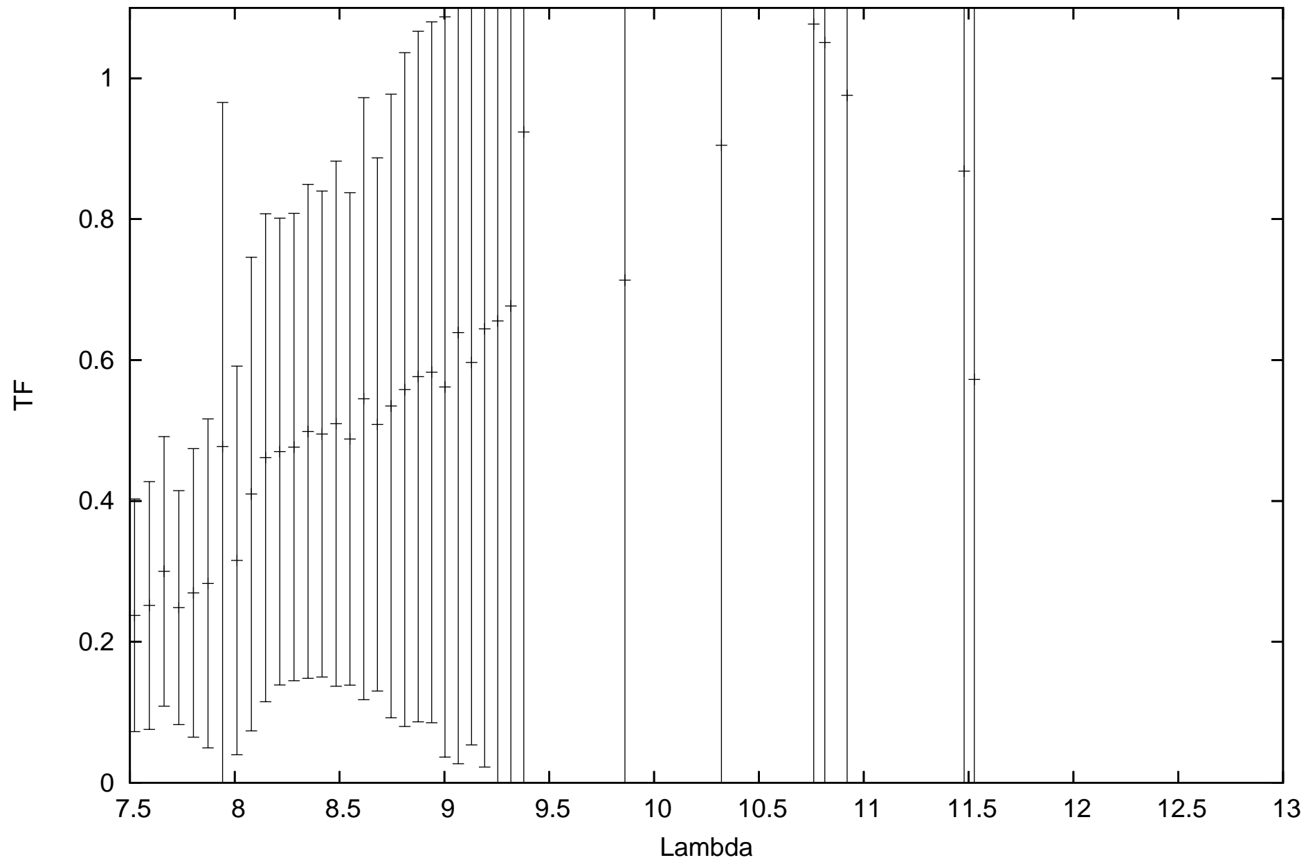
calHD68553_flux0.59_diam3.8_r.MIDI.2011-10-04T08_30_50.000_K0J3
