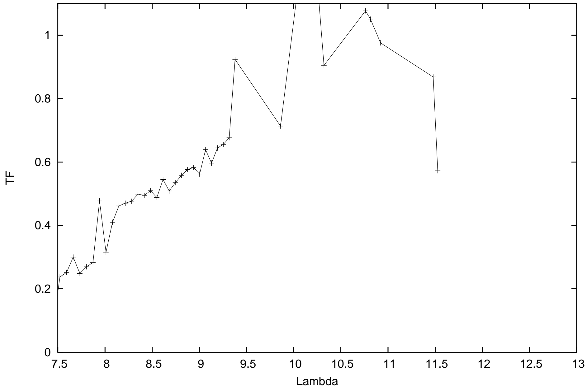
calHD68553_flux0.59_diam3.8_r.MIDI.2011-10-04T08_30_50.000_K0J3
