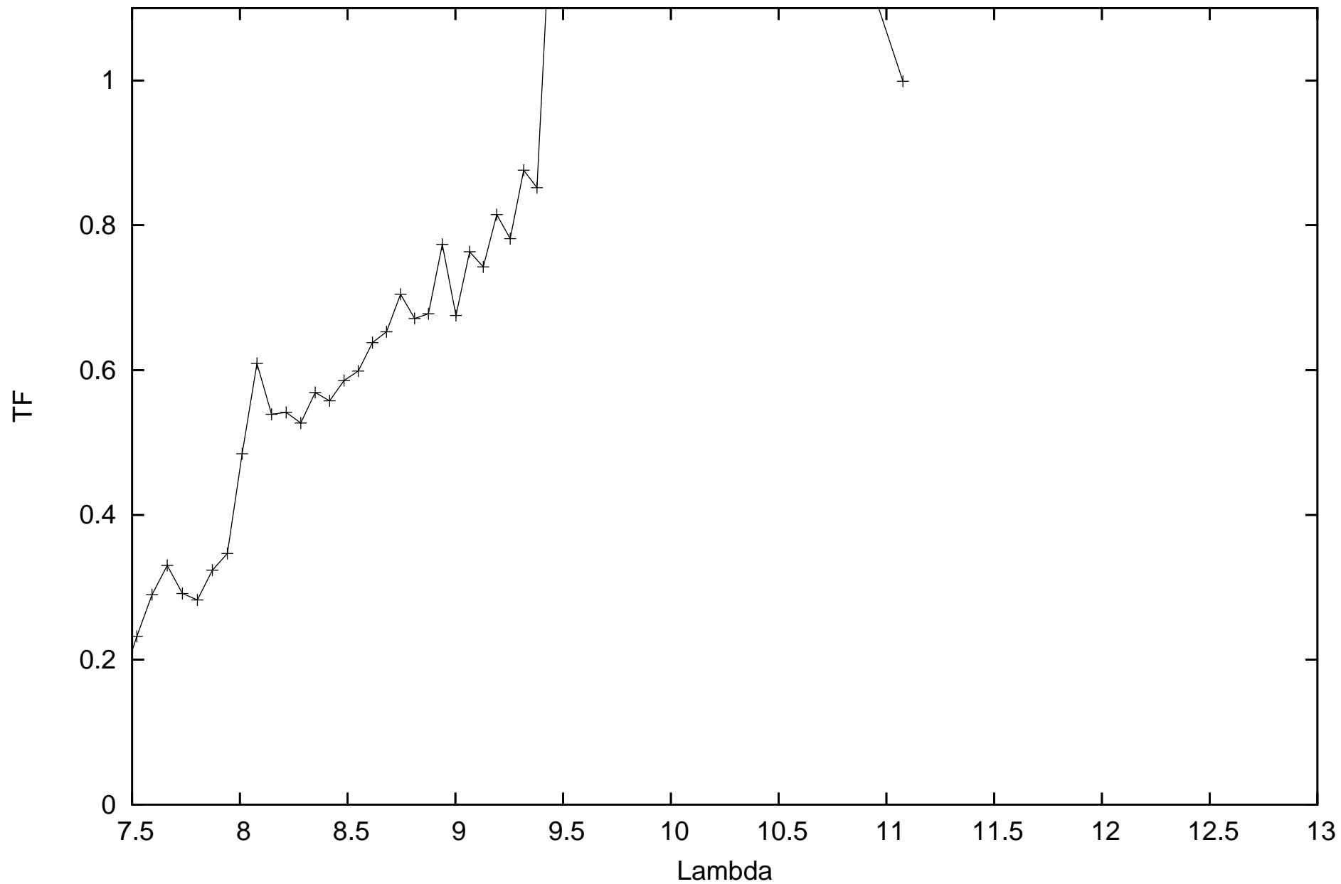
calHD68553_flux0.59_diam3.8_r.MIDI.2011-10-04T08_14_27.000_J3K0
