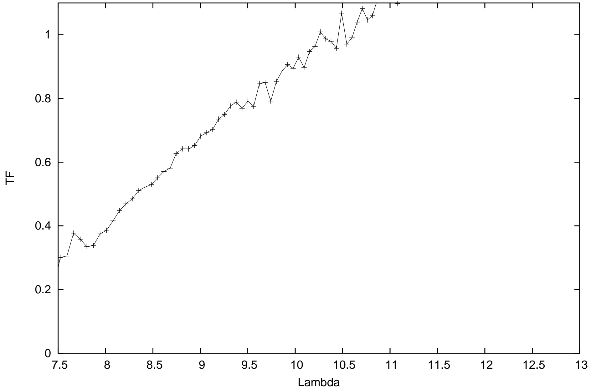
calHD20720_flux-1.53_diam10.14_r.MIDI.2011-10-04T09_07_59.000_J3A1
