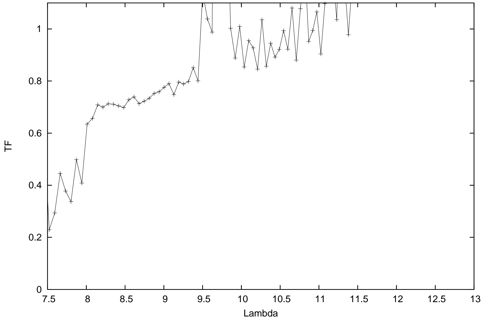
calHIP33357_flux0.277058_diam4.37_r.MIDI.2011-10-03T07_25_09.000_G1J3
