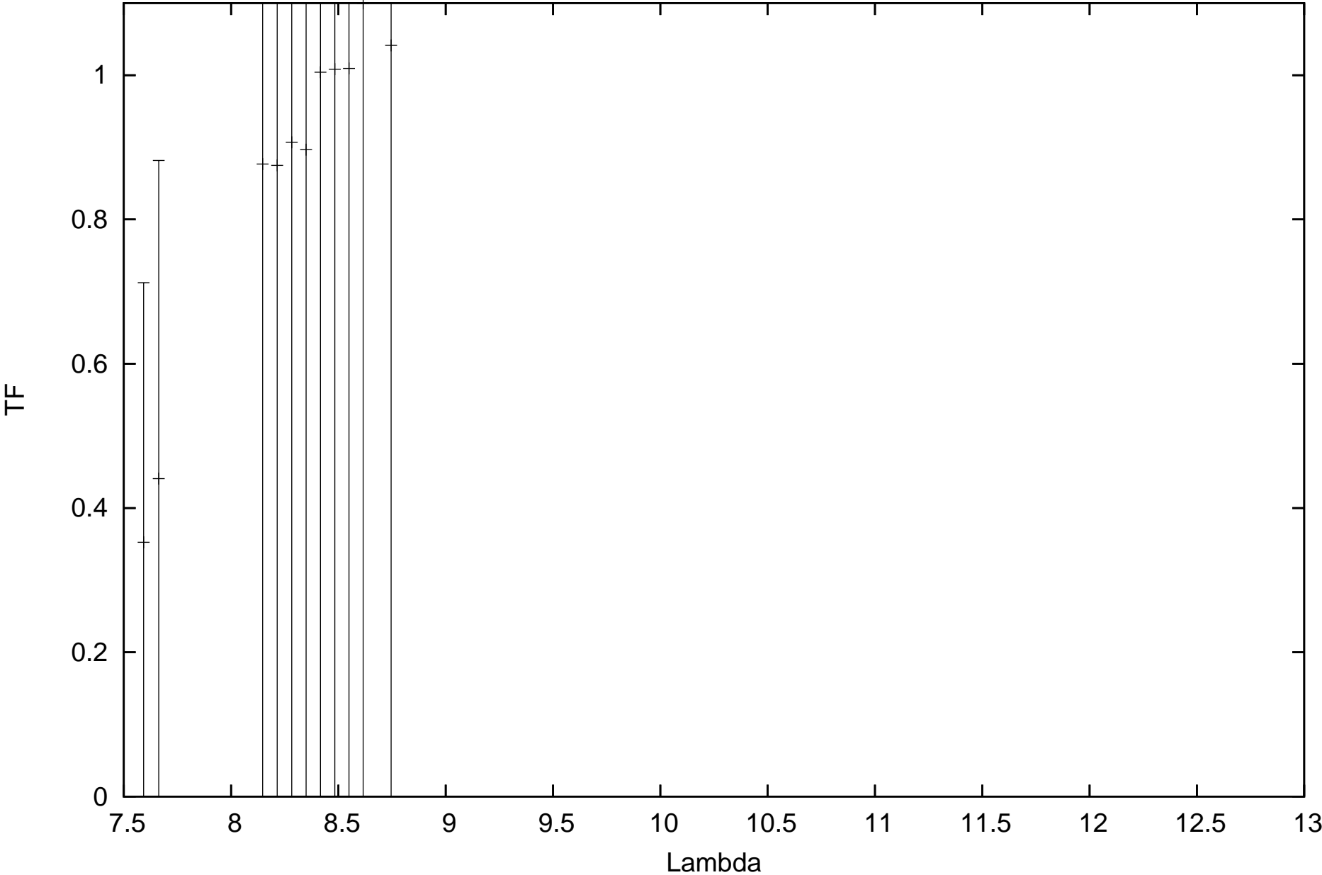
calHIP33357_flux0.277058_diam4.37_r.MIDI.2011-10-03T07_06_58.000_J3G1
