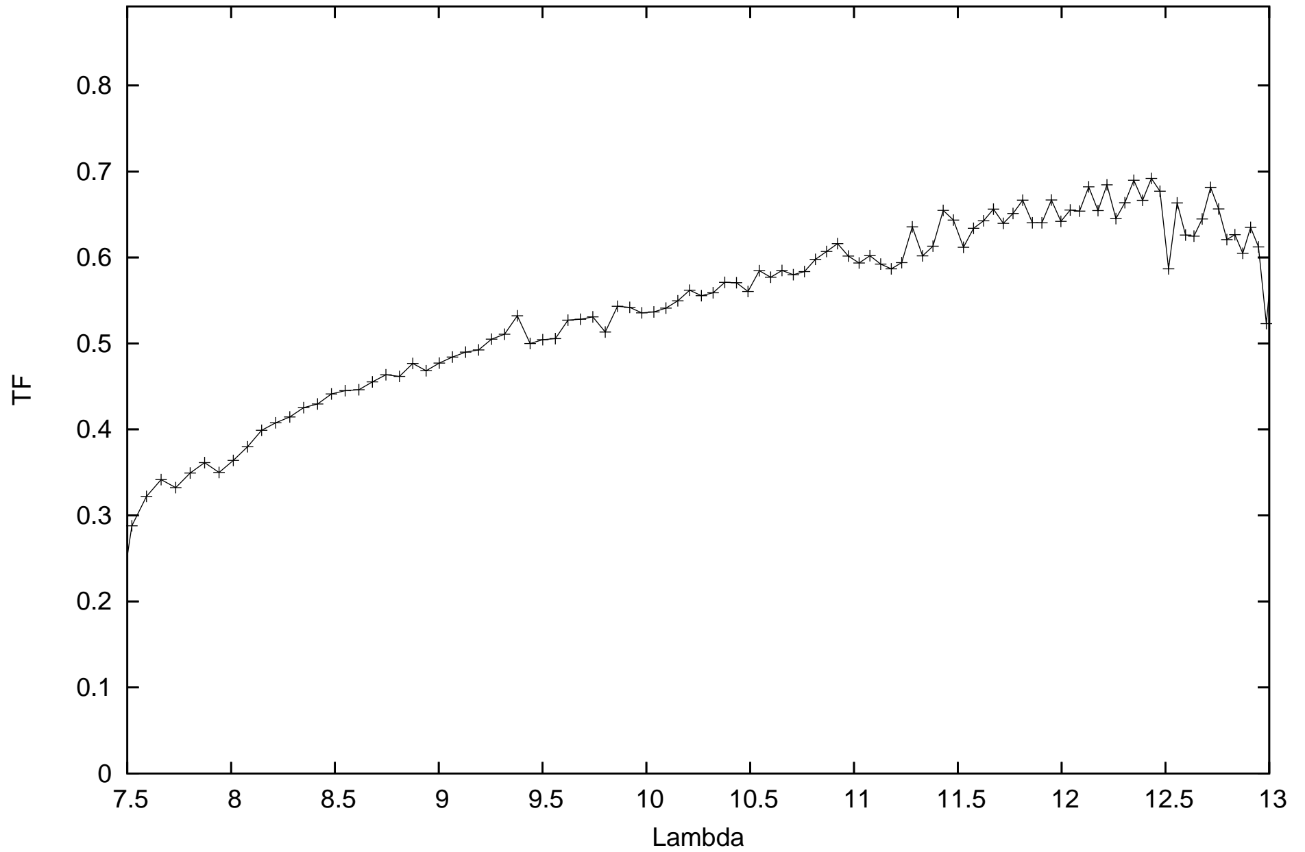
calHD206778_flux-1.04_diam7.59_r.MIDI.2011-10-03T03_15_44.000_J3A1
