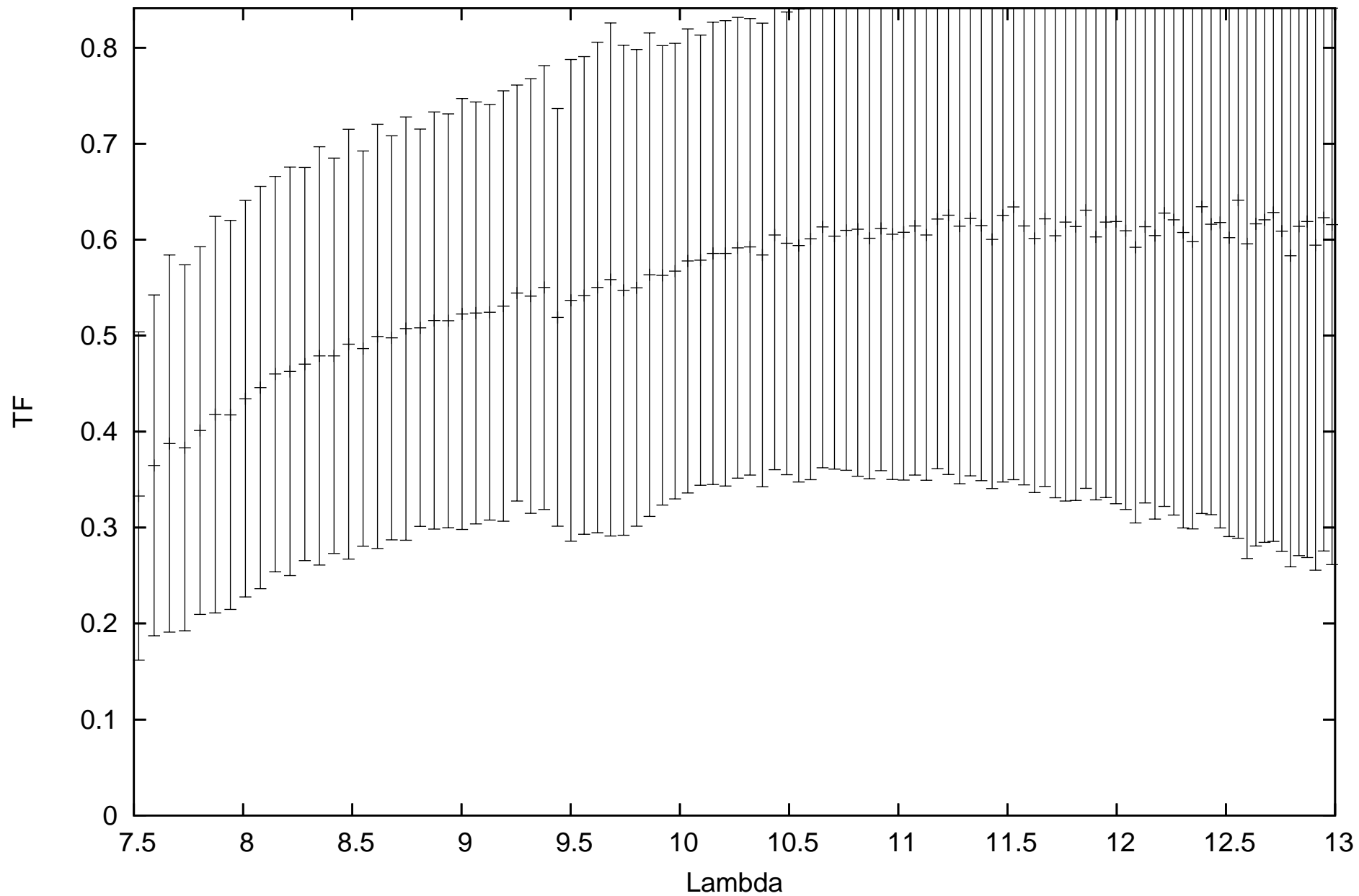
calHD167618_flux-1.82_diam11.66_r.MIDI.2011-10-01T01_30_36.000_G1A1
