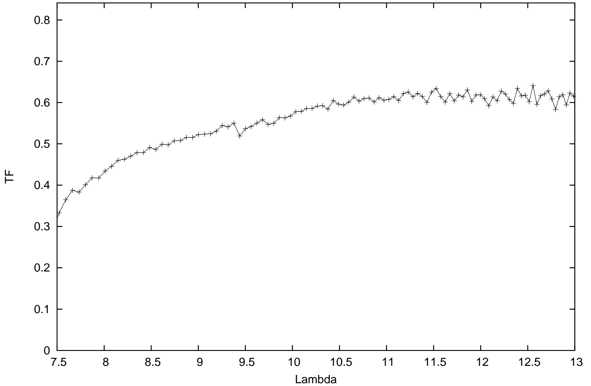
calHD167618_flux-1.82_diam11.66_r.MIDI.2011-10-01T01_30_36.000_G1A1
