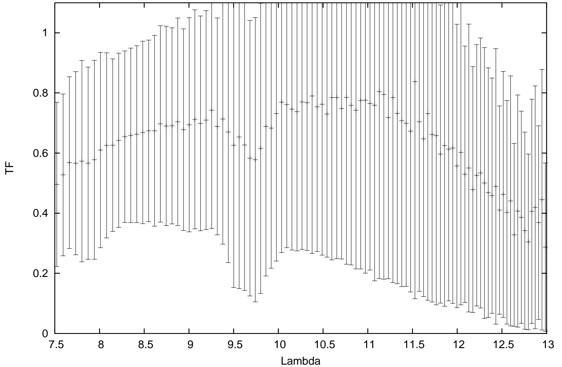
calHD152161_flux-0.26_diam6.12_r.MIDI.2011-09-22T00_26_17.000_G1A1
