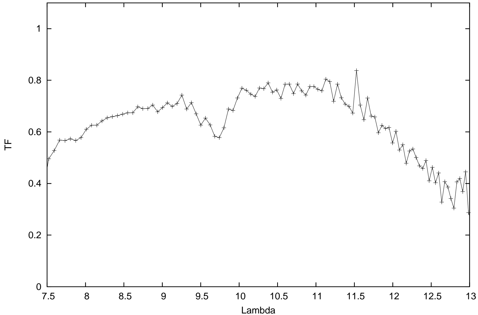
calHD152161_flux-0.26_diam6.12_r.MIDI.2011-09-22T00_26_17.000_G1A1
