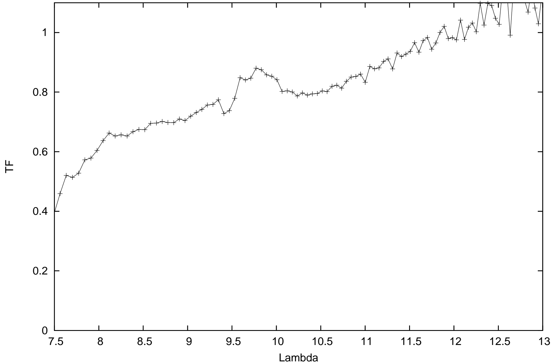
calHIP112748_flux1.25758_diam2.46_r.MIDI.2011-09-14T04_05_01.128_U3U4
