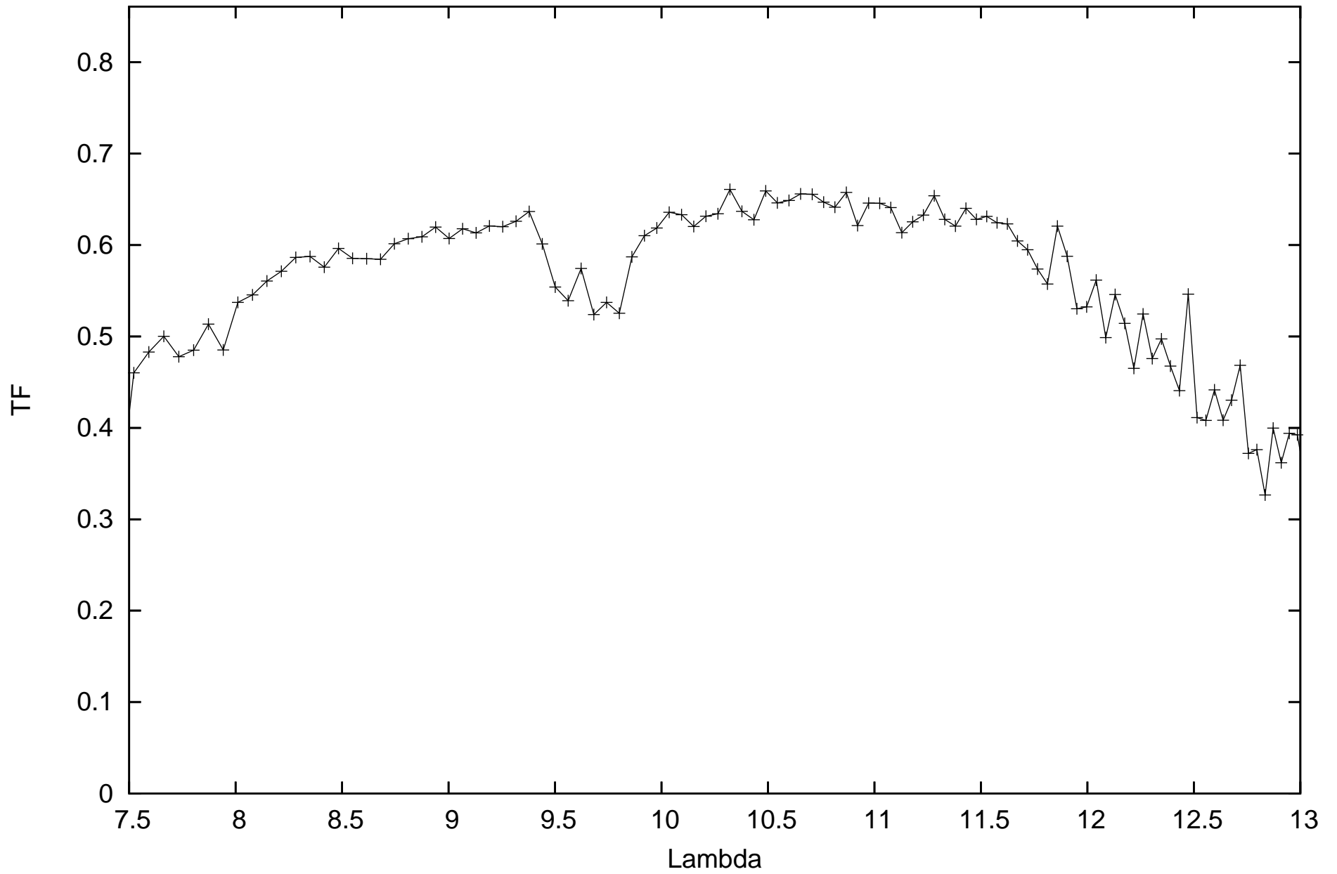
calHIP1170_flux-0.10766_diam5.17_r.MIDI.2011-09-13T06_19_07.000_A1J3
