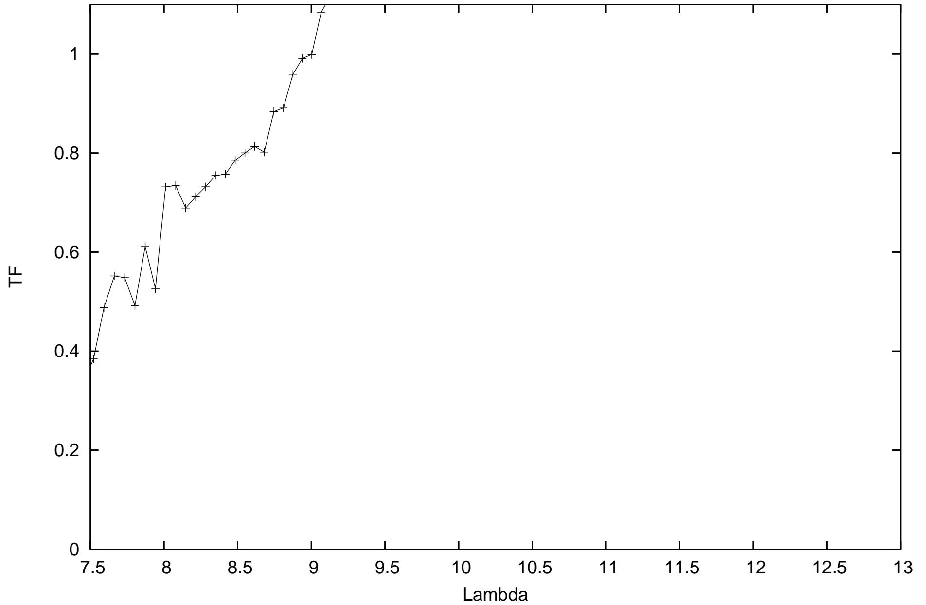
calHD33684_flux0.03_diam5.07_r.MIDI.2011-09-13T08_23_34.000_K0A1
