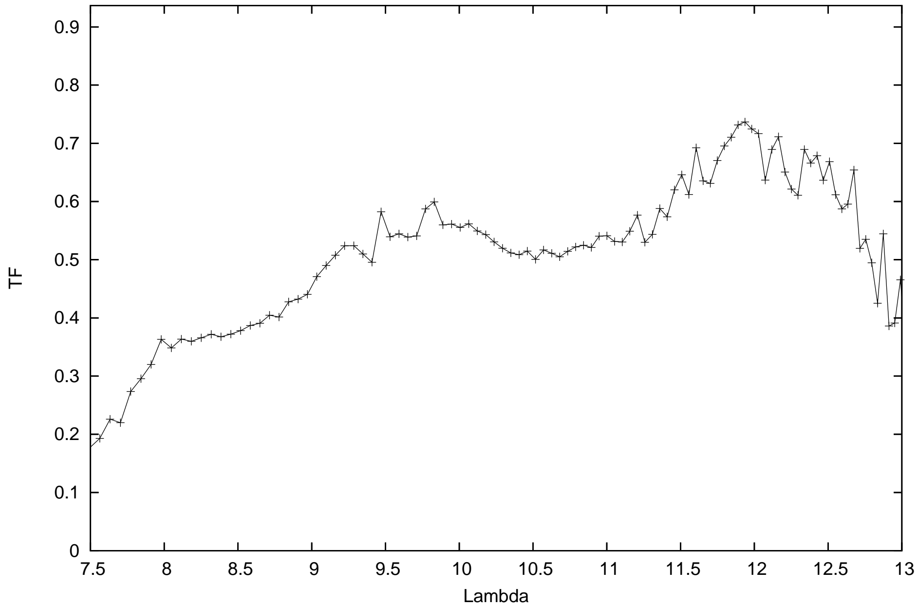
calHIP73714_flux-1.78451_diam11.15_r.MIDI.2011-08-29T00_49_21.940_I1A1
